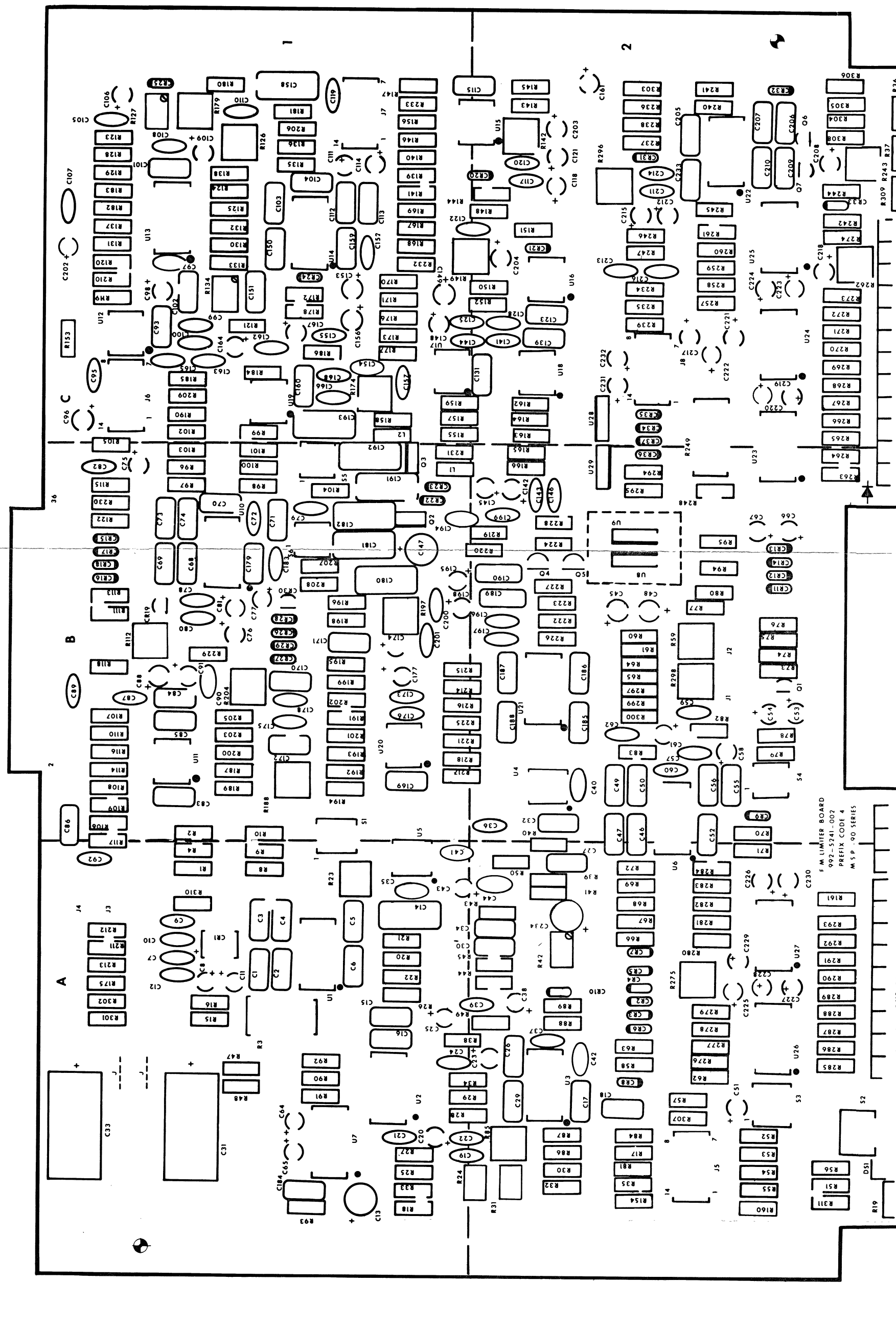
1899-21 FIGURE 3-2. FM LIMITER MODULE ELECTRICAL COMPONENTS LOCATION
