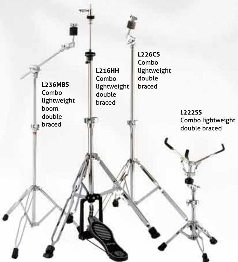
L422SS 400 series double braced
