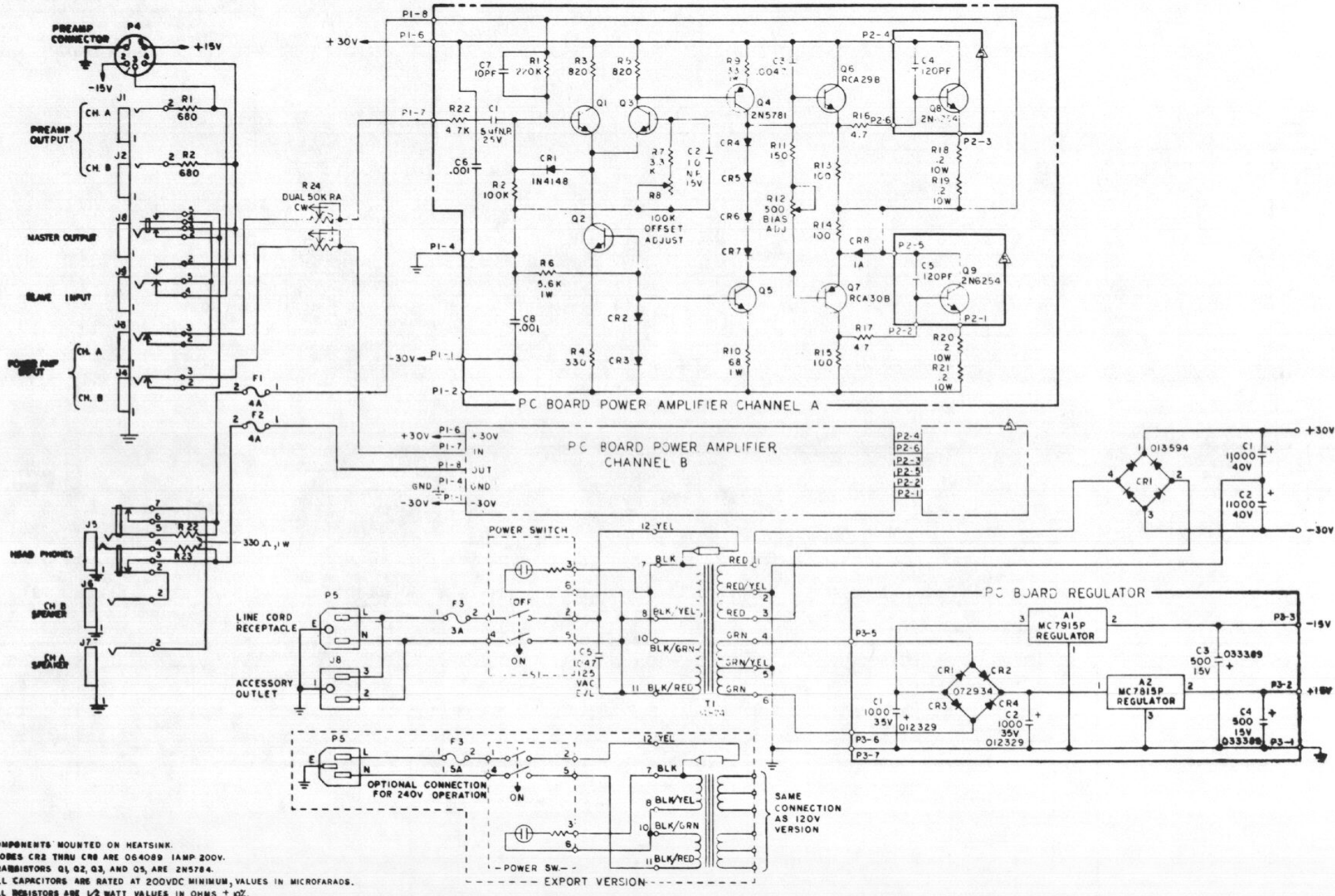
Figure 11-4. Schematic — Power Amplifier — Janus I
