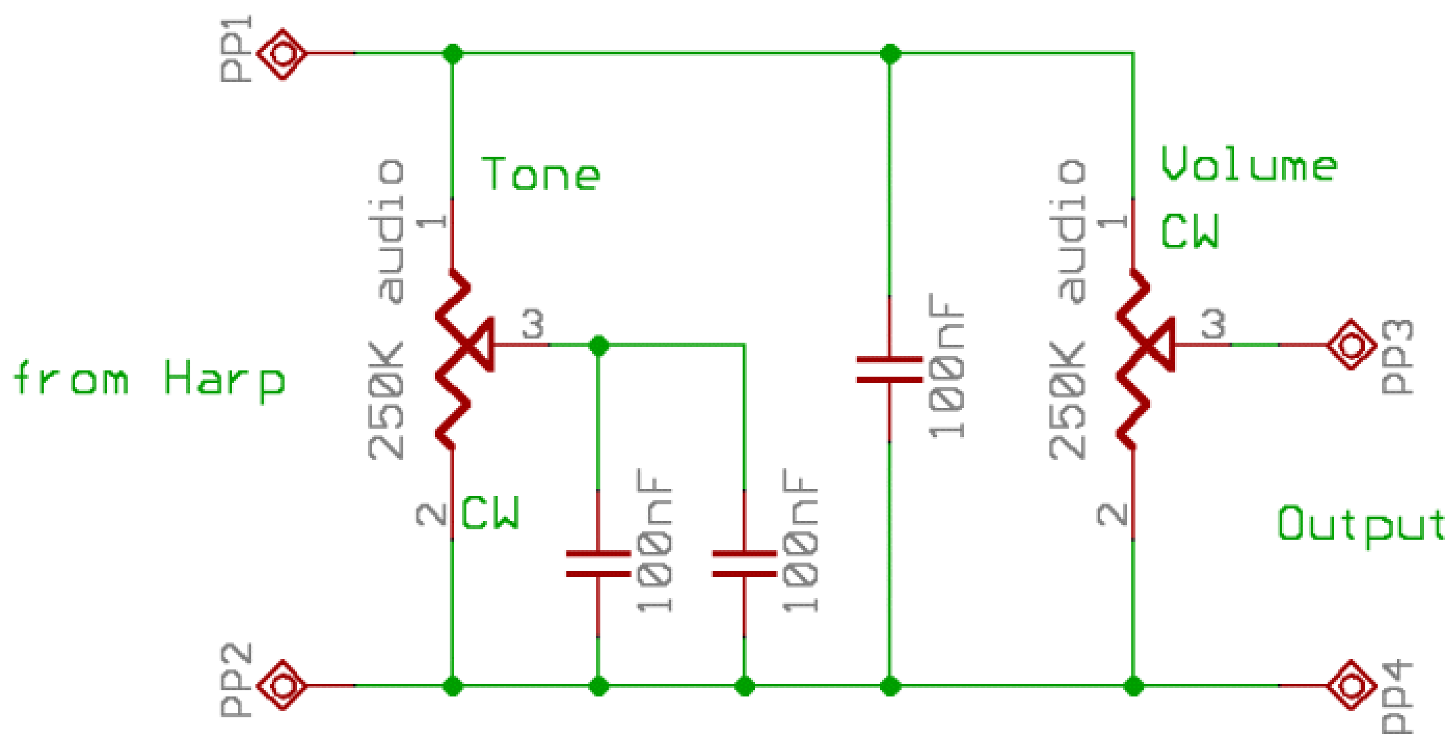
Piano Bass schematic
