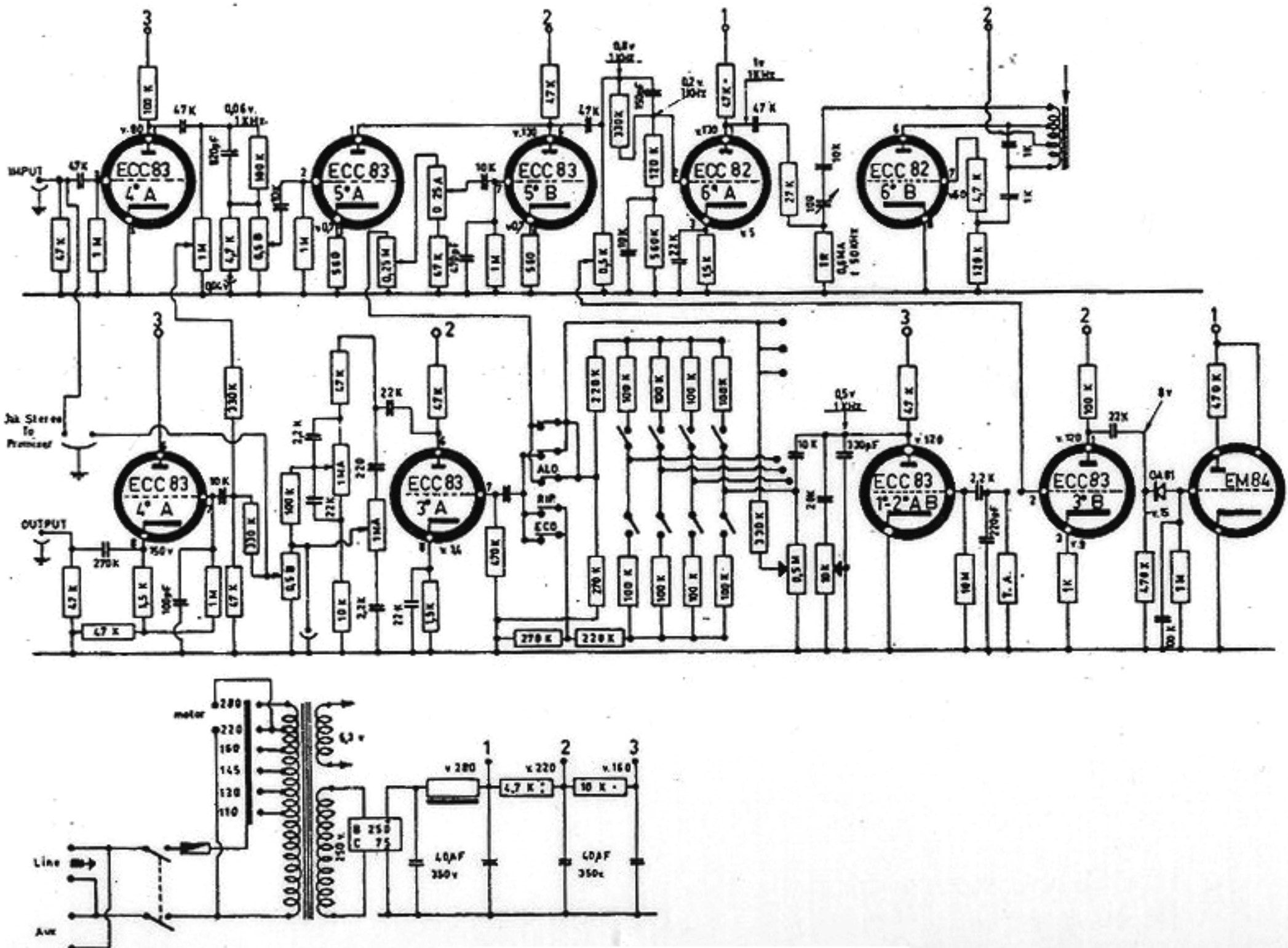
Wiring diagram of the P.E. 603-T Echorec
