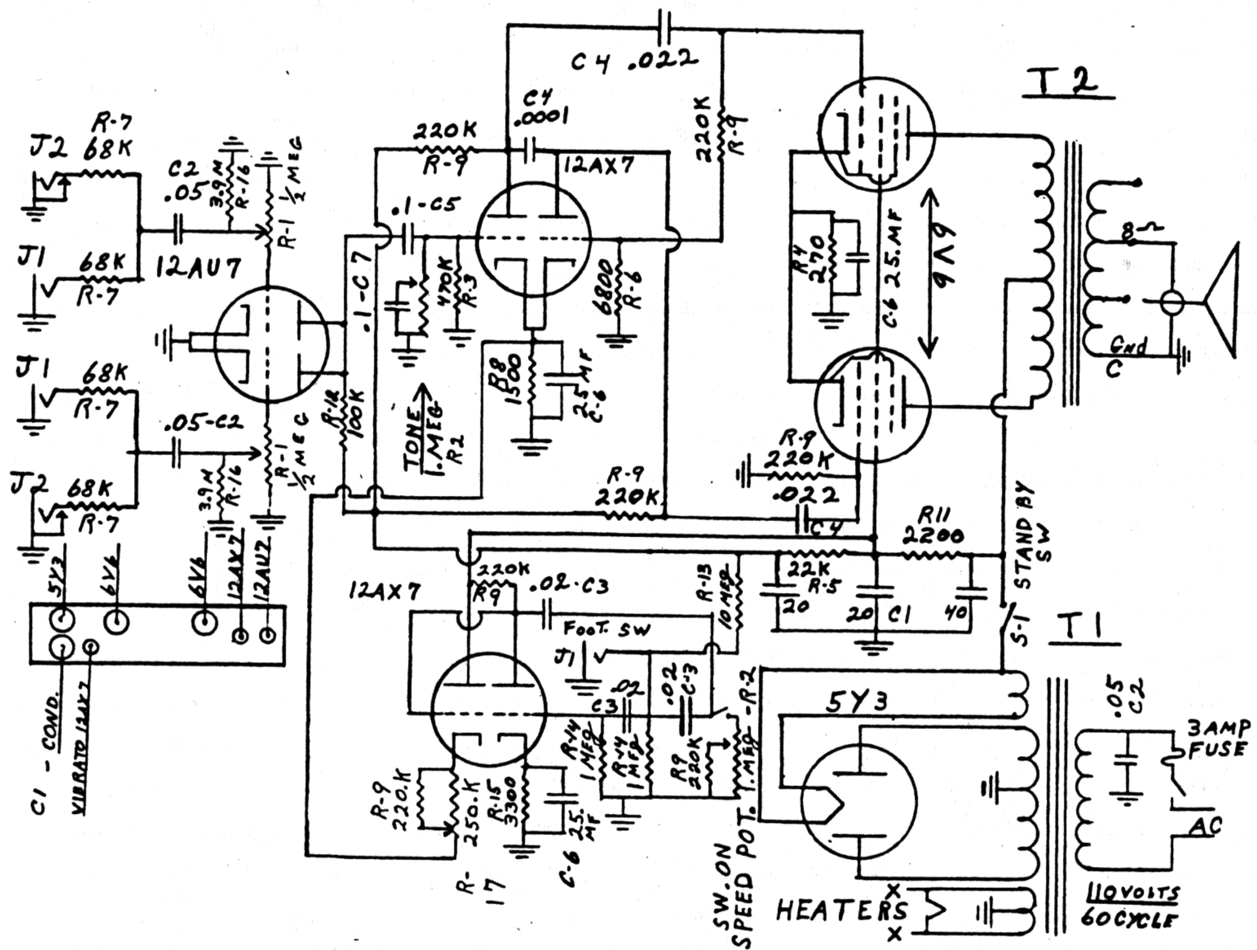
Key Model 506
