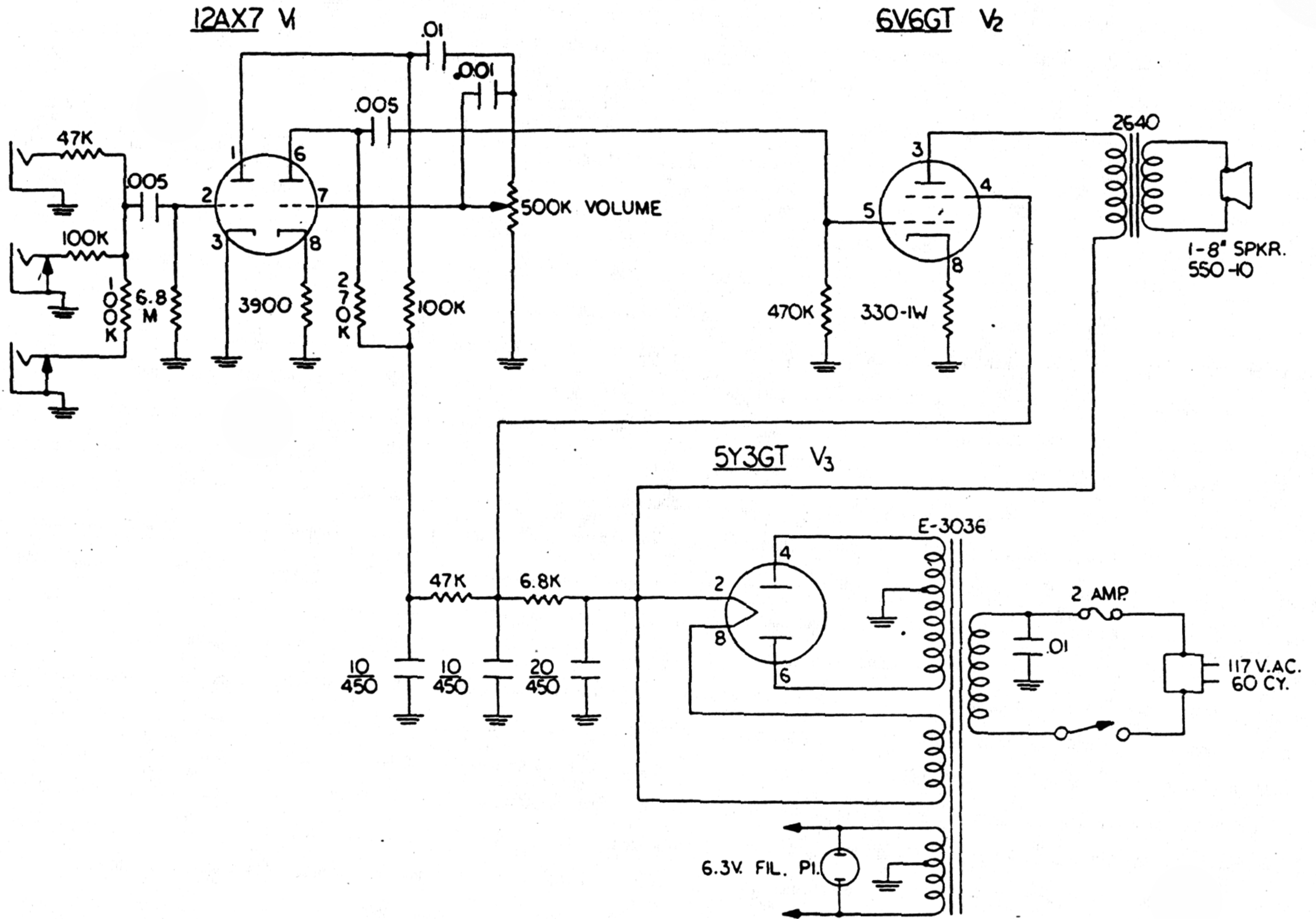
Valco Model 6150
