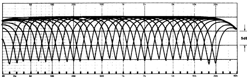
Cut Only 1/3 Octave Equaliser Filter Curves.
