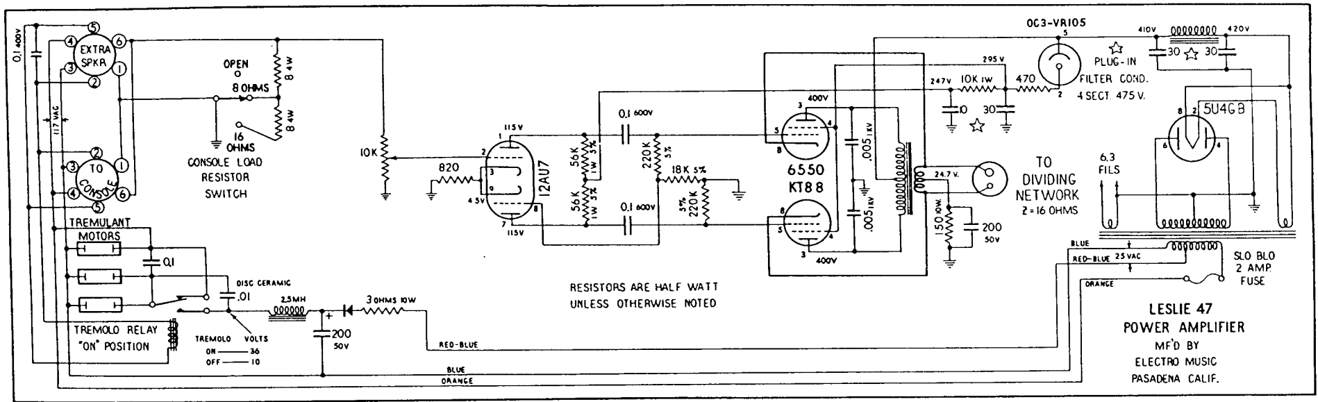
ABOVE: Schematic applies to amplifiers in Model 45 Speakers below serial 61400, and to Model 47 Speakers below serial 82800.
