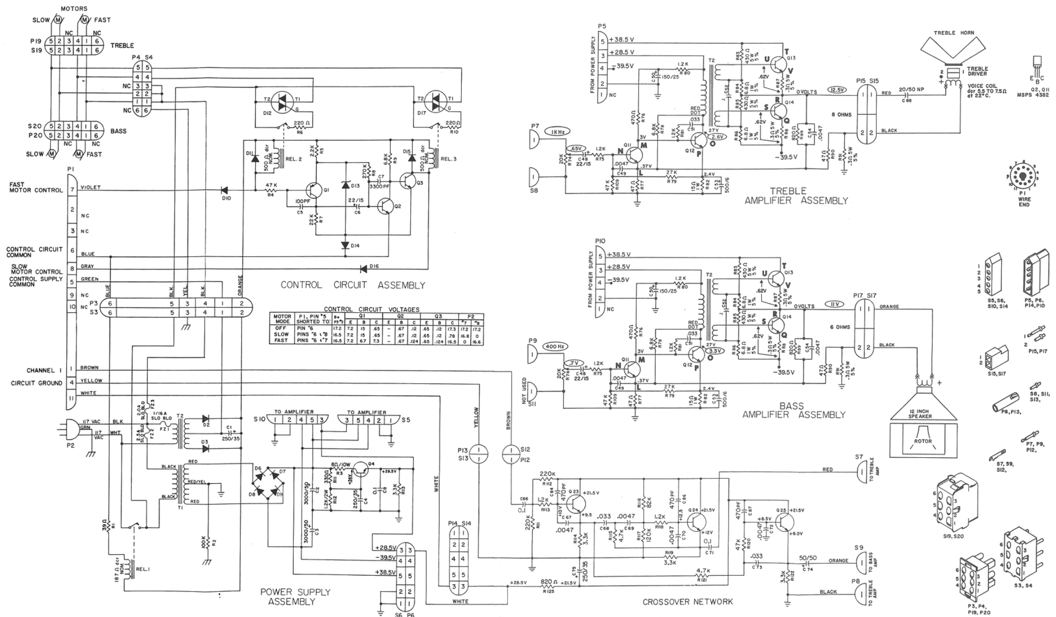
Figure 40. Schematic, LESLIE Speaker Model 860
