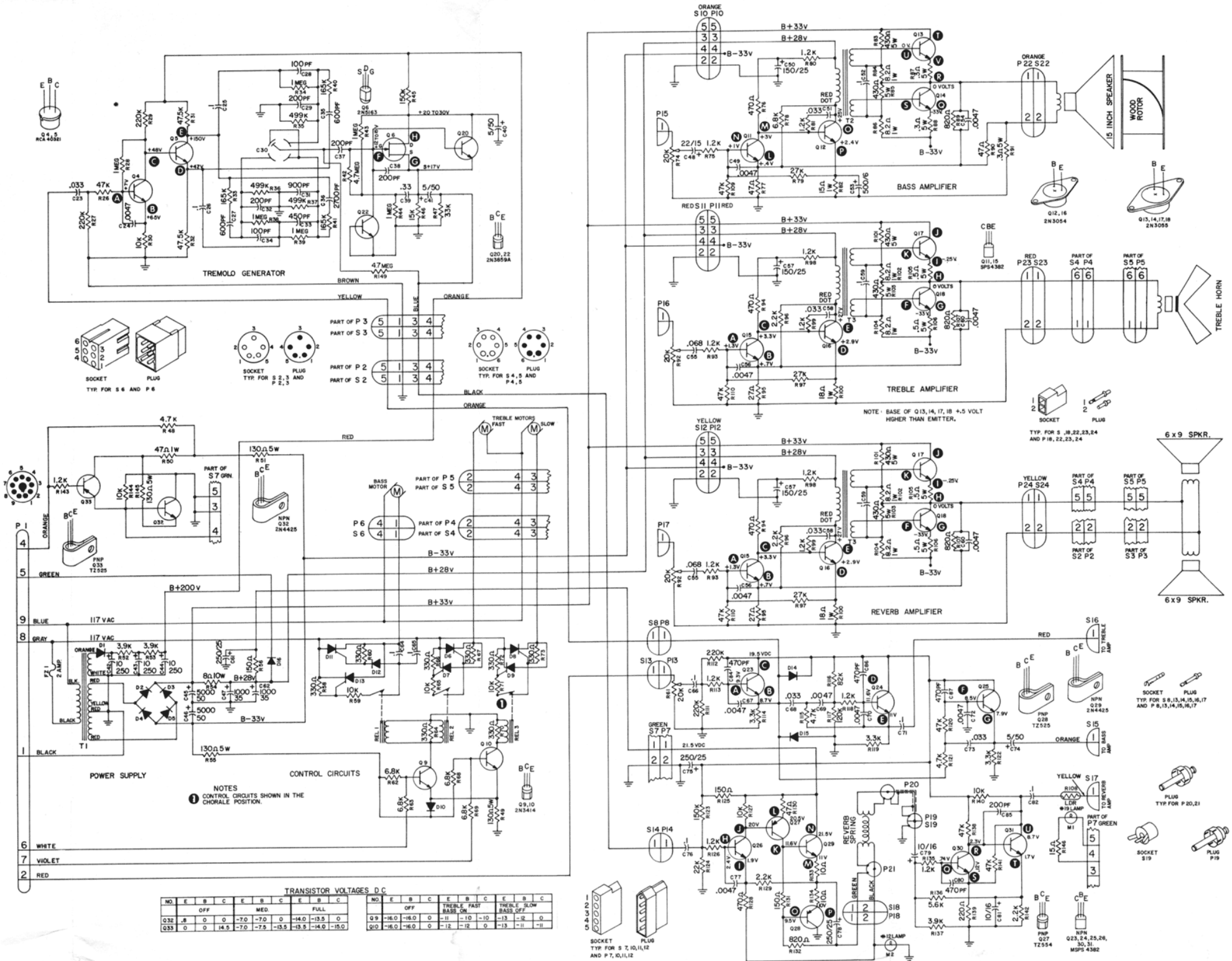
Figure 28. Schematic, LESLIE Speaker Model 910
