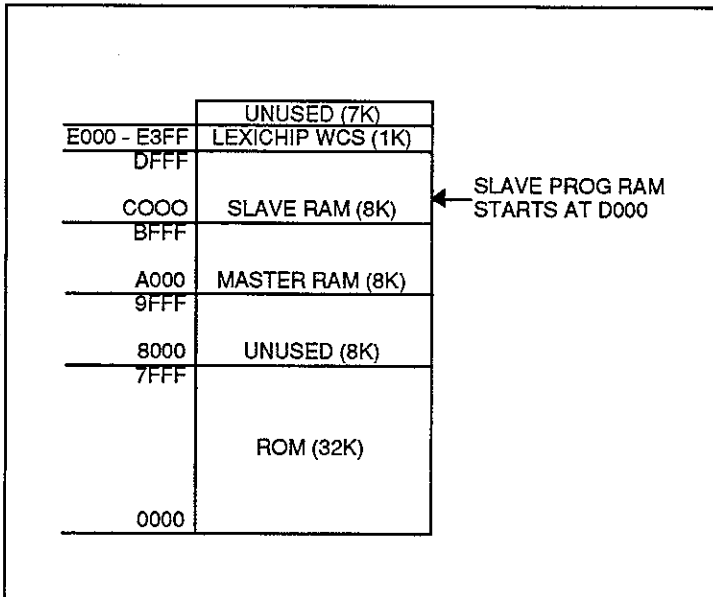
Master Processor Memory Map
