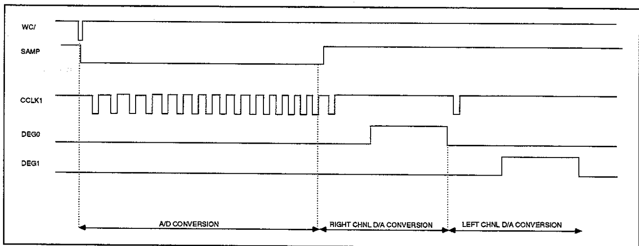
Converter Timing
