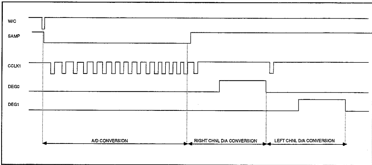
A/D SAR Conversion Timing
