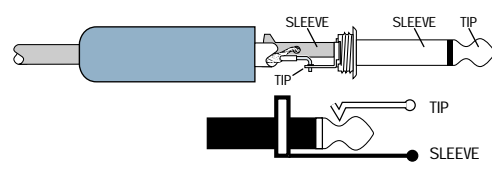
Figure C: TS Plug
