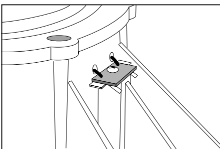
Terminal board of the midrange transducer
