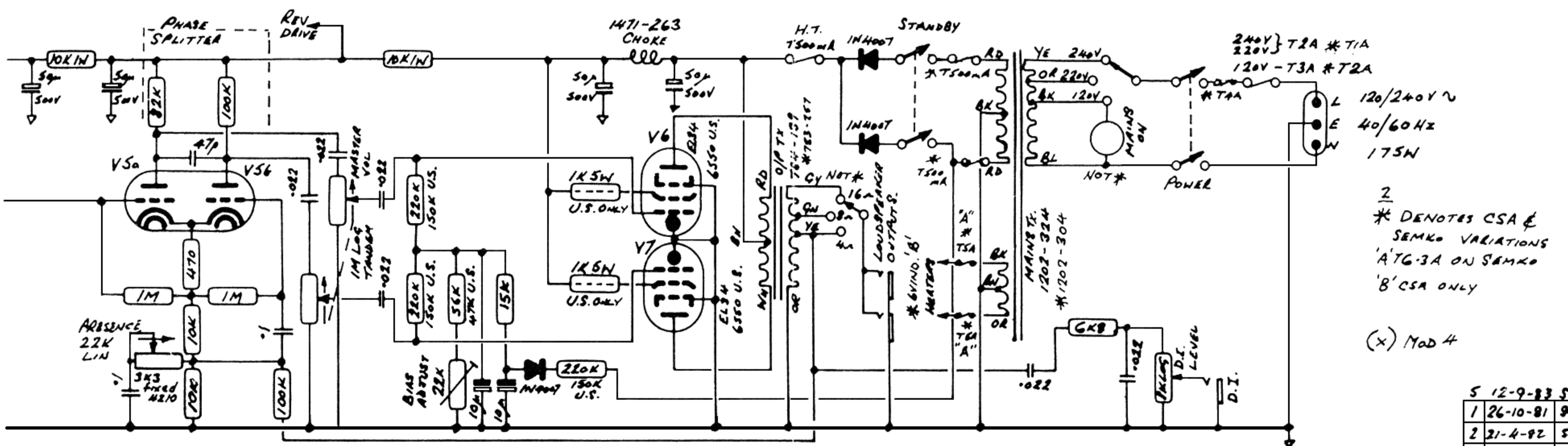
Marshall JCM 800 Series Model 4210 50 W Reverb Combo - Circuit Diagram MODEL 2205 50W AMP HEAD
