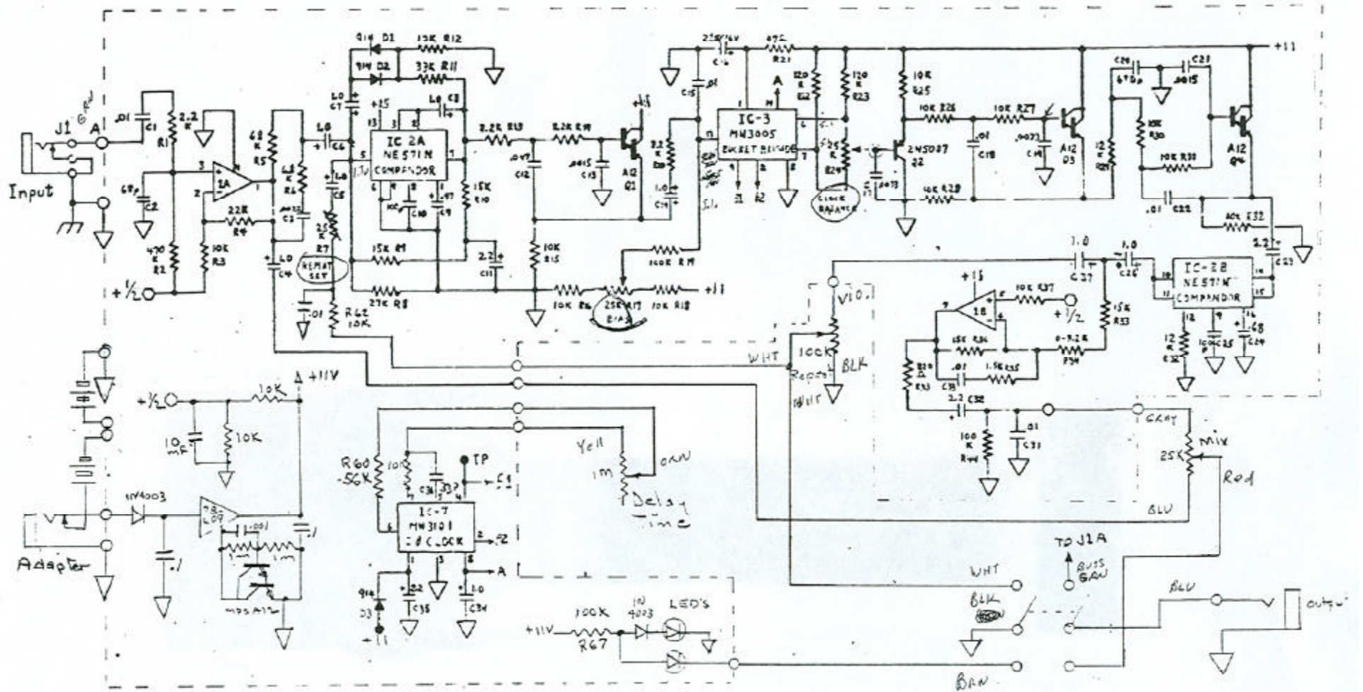
MORLEY AER Analog Echo Reverb
