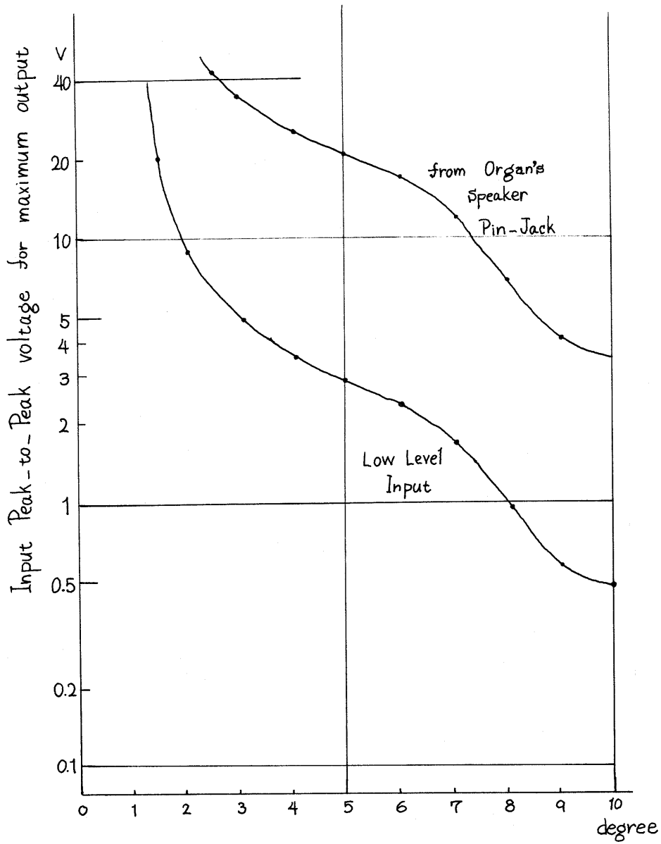
Degree of Balance control
