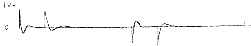
Output of IC11A
