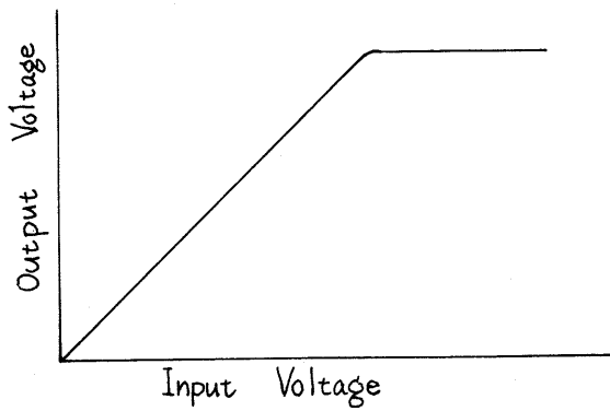
Characteristic of the photo coupler limiter
