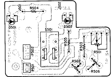
PITCH CONTROL PCB ASSY
