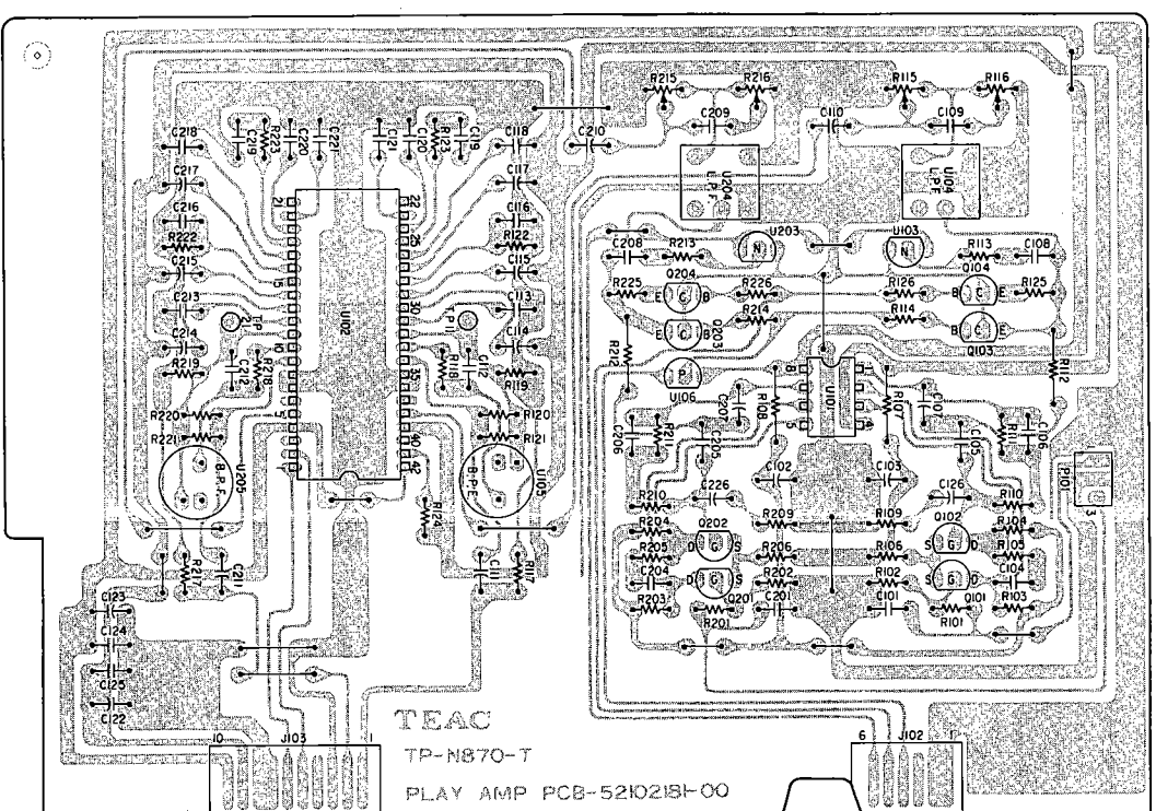
PLAY AMPL PCB ASSY
