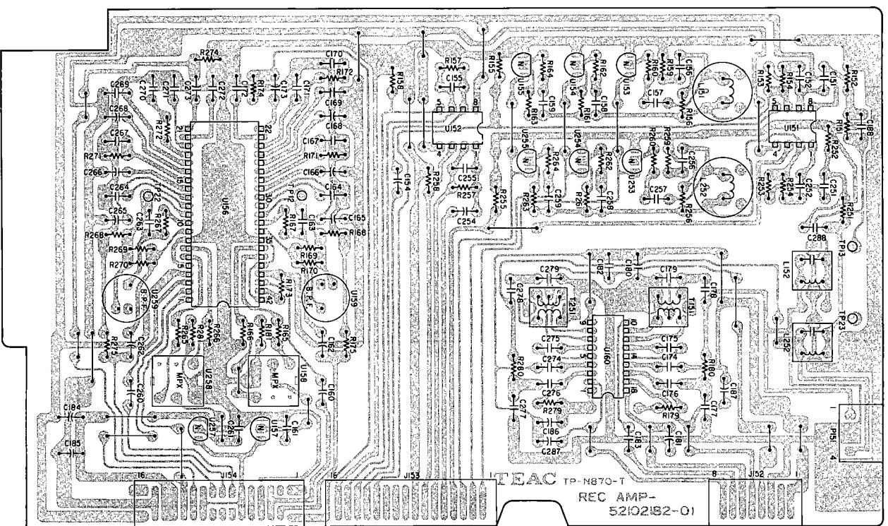
REC AMPL PCB ASSY
