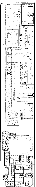
VR PCB ASSY
