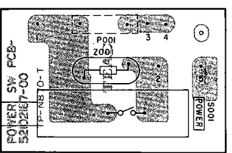
POWER SW PCB ASSY
