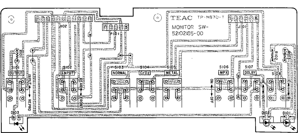
MONITOR SWITCH PCB ASSY
