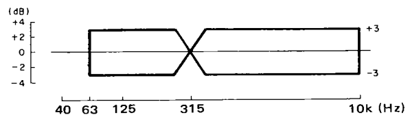
Fig. 6-7 Repr Frequency Response 再生周波数特性
