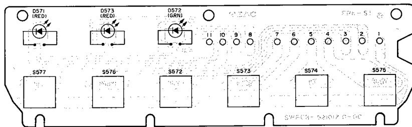
OPERATION SW PCB ASSY
