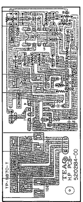
HEADPHONE PCB ASSY
