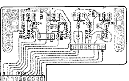
ADJUSTMENT VR PCB ASSY
