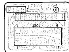
REMOTE CONNECTOR PCB ASSY
