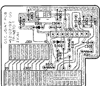
ADJUSTMENT SW PCB ASSY
