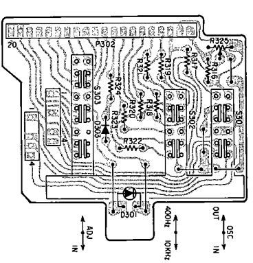
ADJUSTMENT SW PCB ASSY
