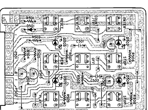
ADJUSTMENT VR PCB ASSY
