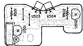
SENSOR PCB ASSY
