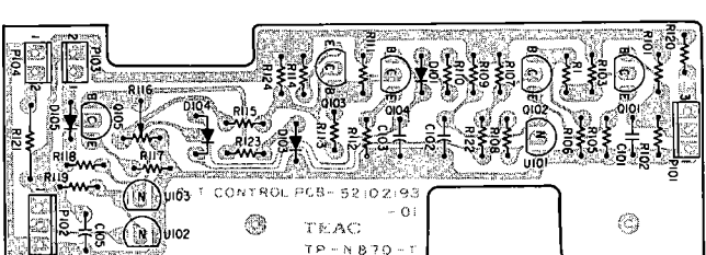
B.T. CONTROL PCB ASSY
