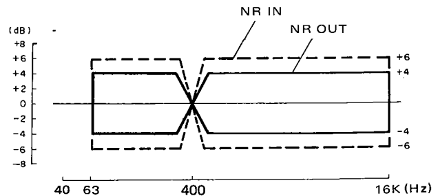
Fig. 6-12 Overall Frequency Response 総合周波数特性
