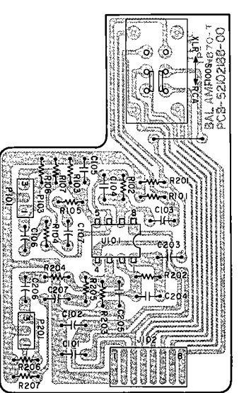
BAL. AMPL PCB ASSY
