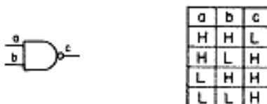
(a) 2 INPUT NAND GATE
