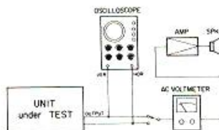
Fig. 2-10. Head Azimuth Test Set-Up
