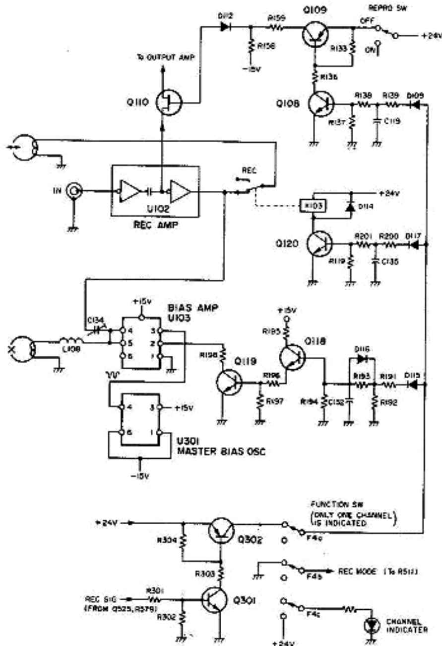
Fig. 1-15 (A). Bias and Record Control Circuit
