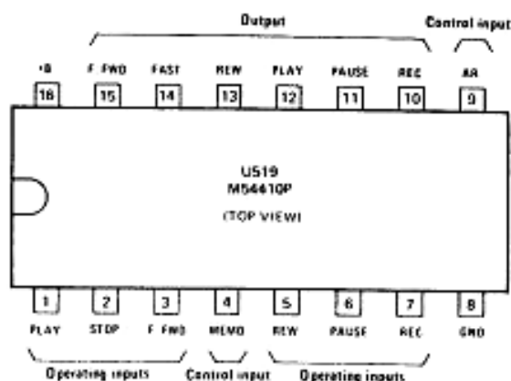
Fig. 1-1. Pin Assignments
