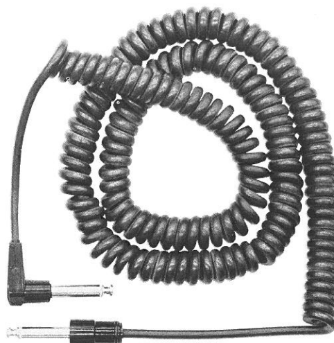
COIL CORD: V841 RED, V842 GREEN, V843 YELLOW, V844 WHITE, V845 BLACK
