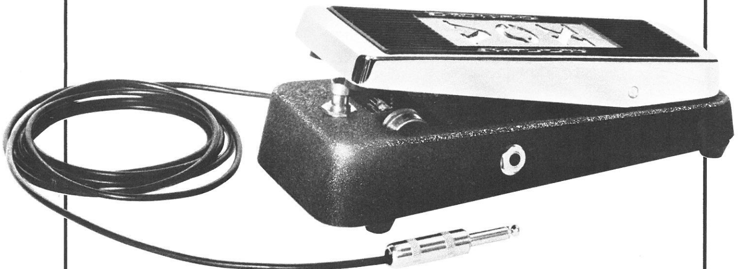
WAH-WAH PEDAL: V846
