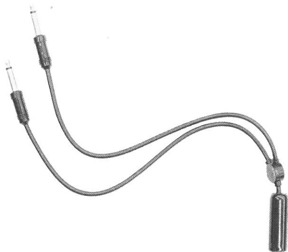
Y-ADAPTER CORD: V824
