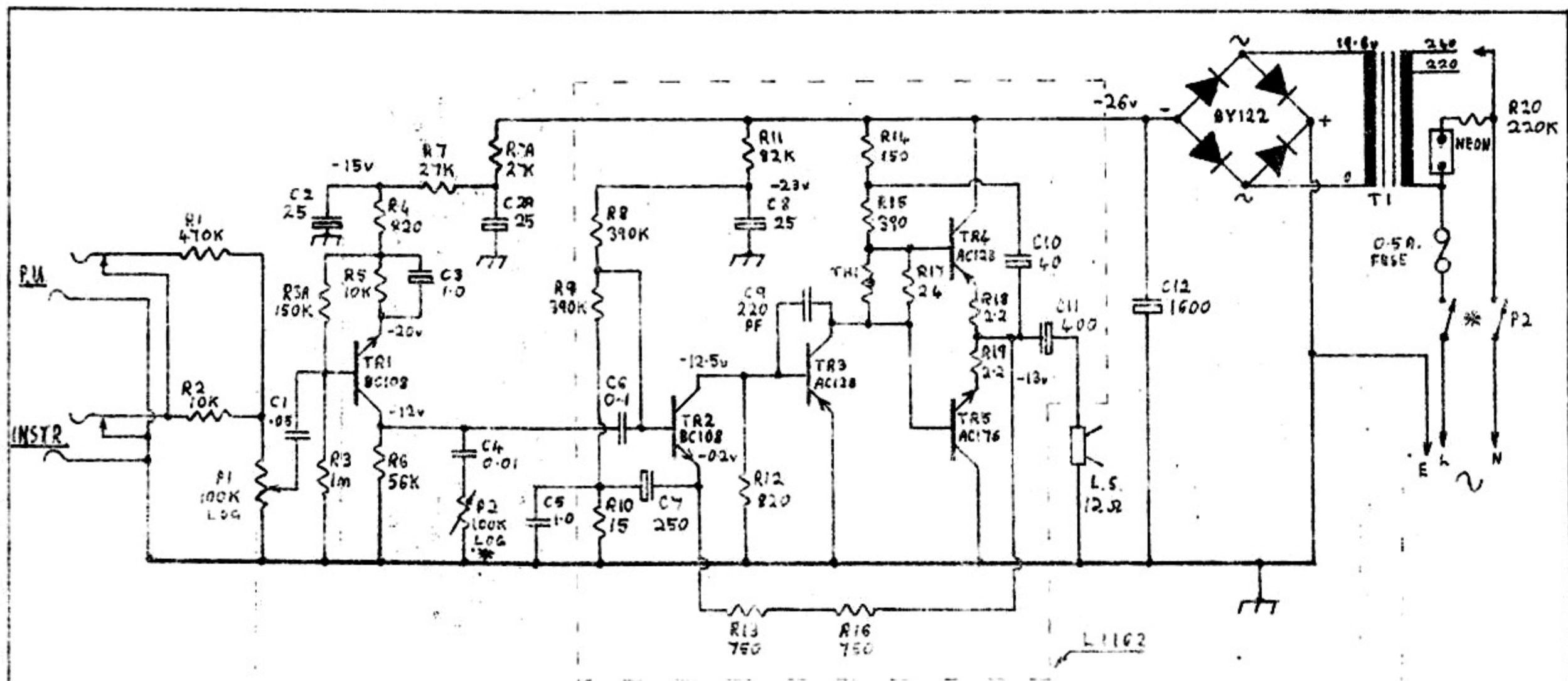
CIRCUIT CLUBMAN SOLID-STATE
