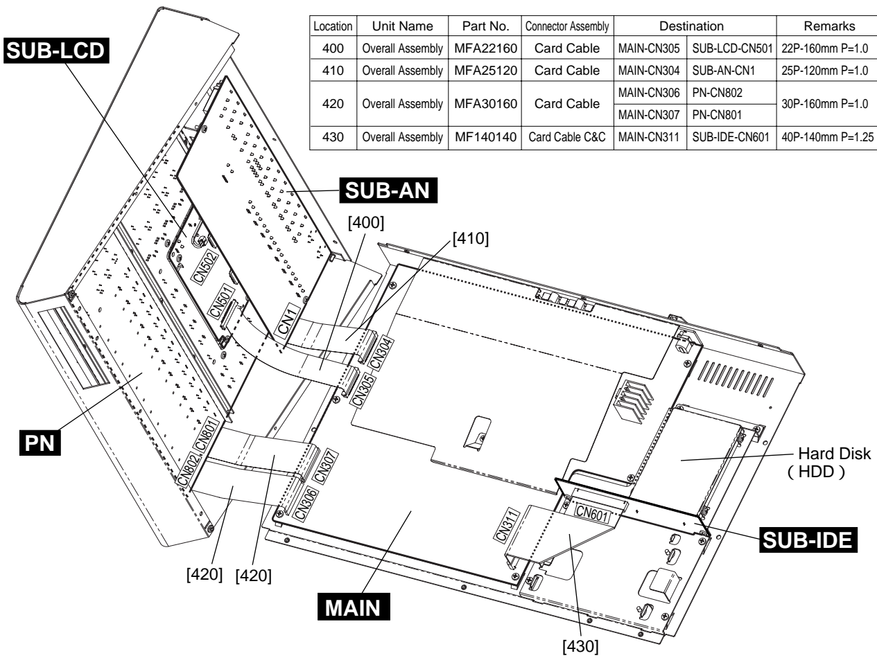
• Top view (Bottom cover section)
