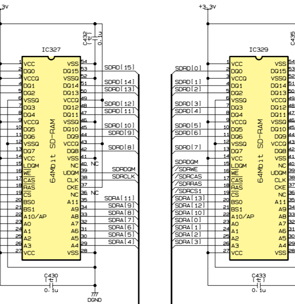
SDRAM 64M
