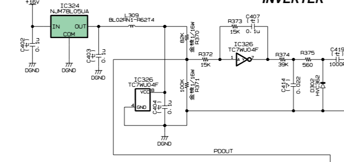
REGULATOR +5V
