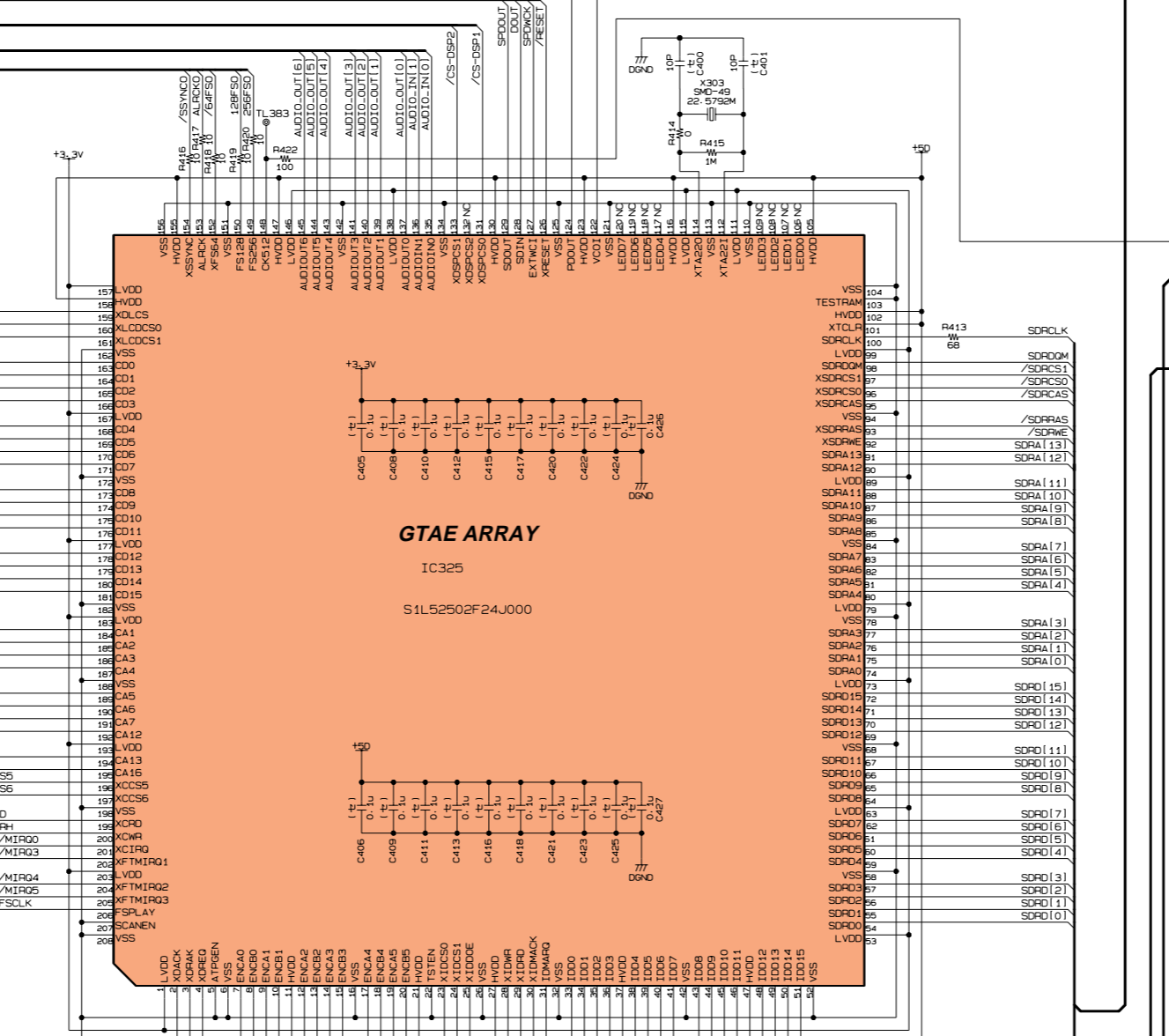
to SUB-IDE-CN601
