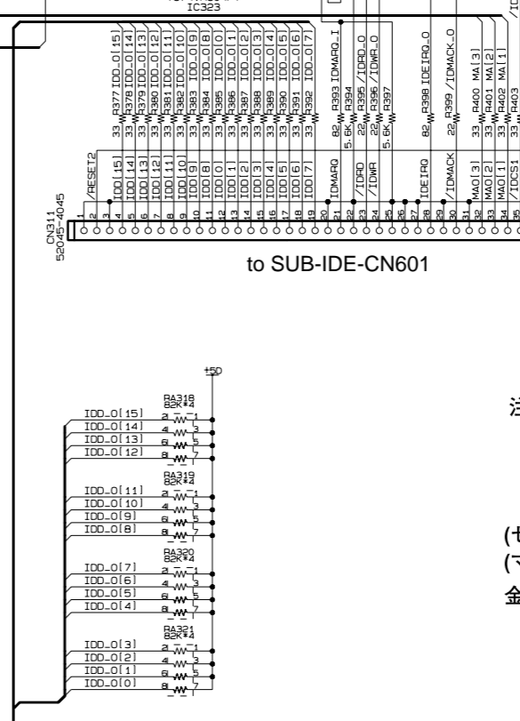
to SUB-IDE-CN601
