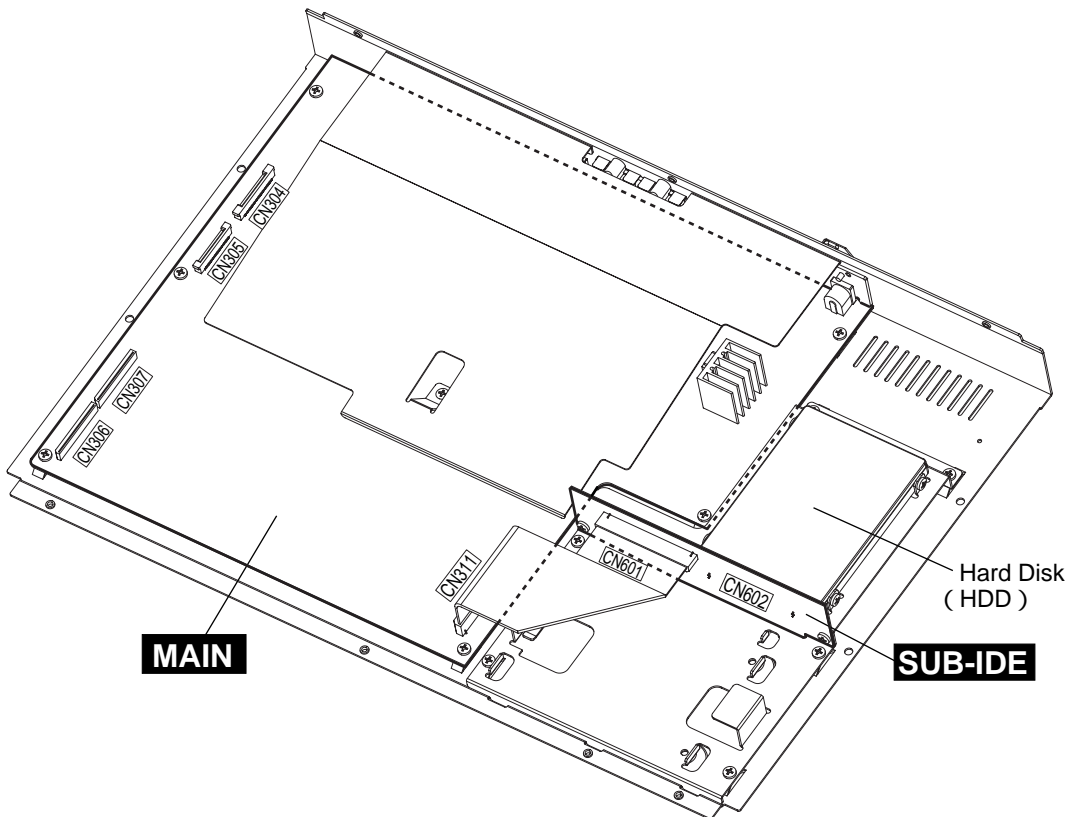
• Top view (Bottom cover section)
