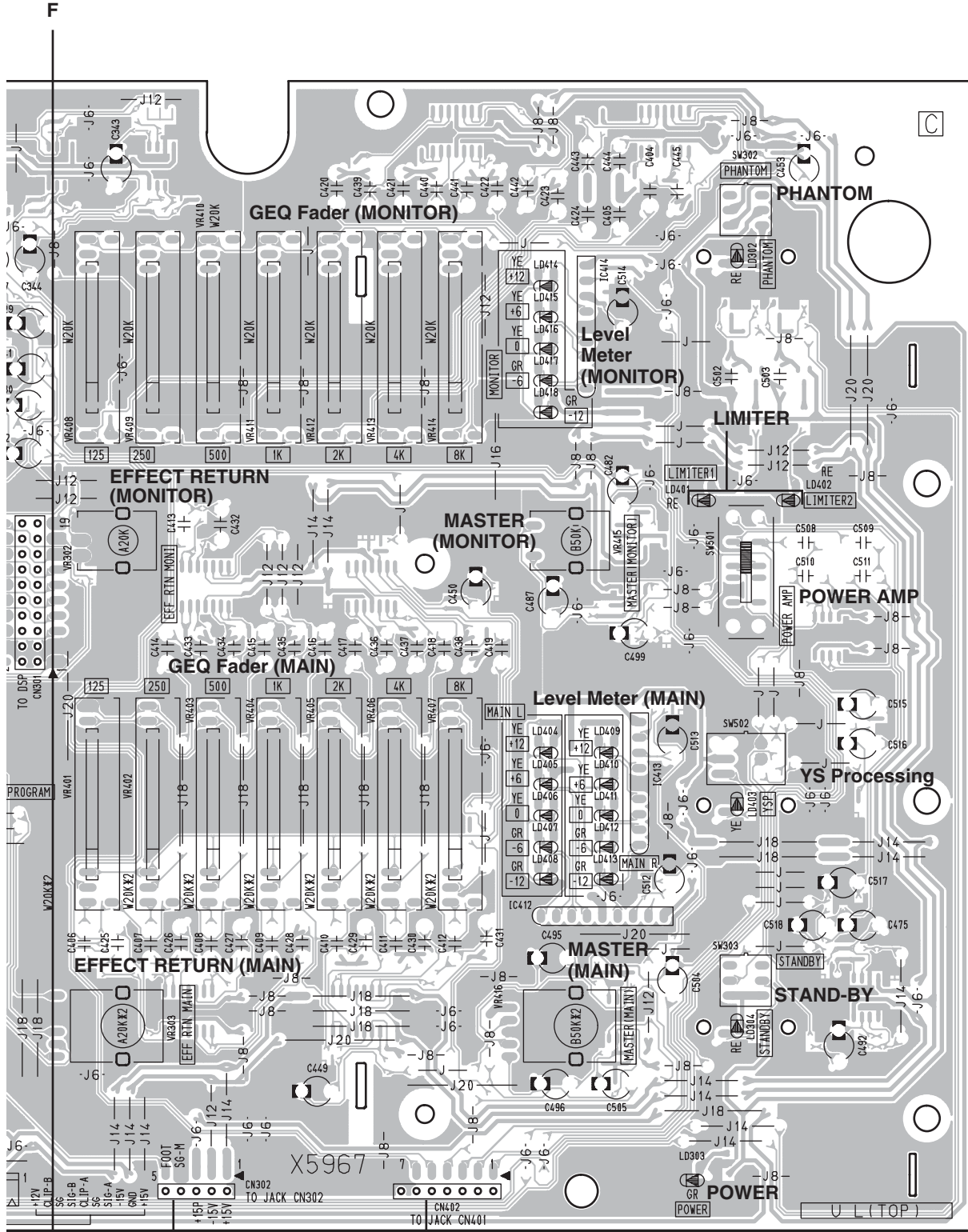
Component side (部品側)
