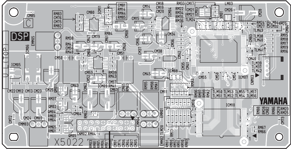
Component side (部品側)
