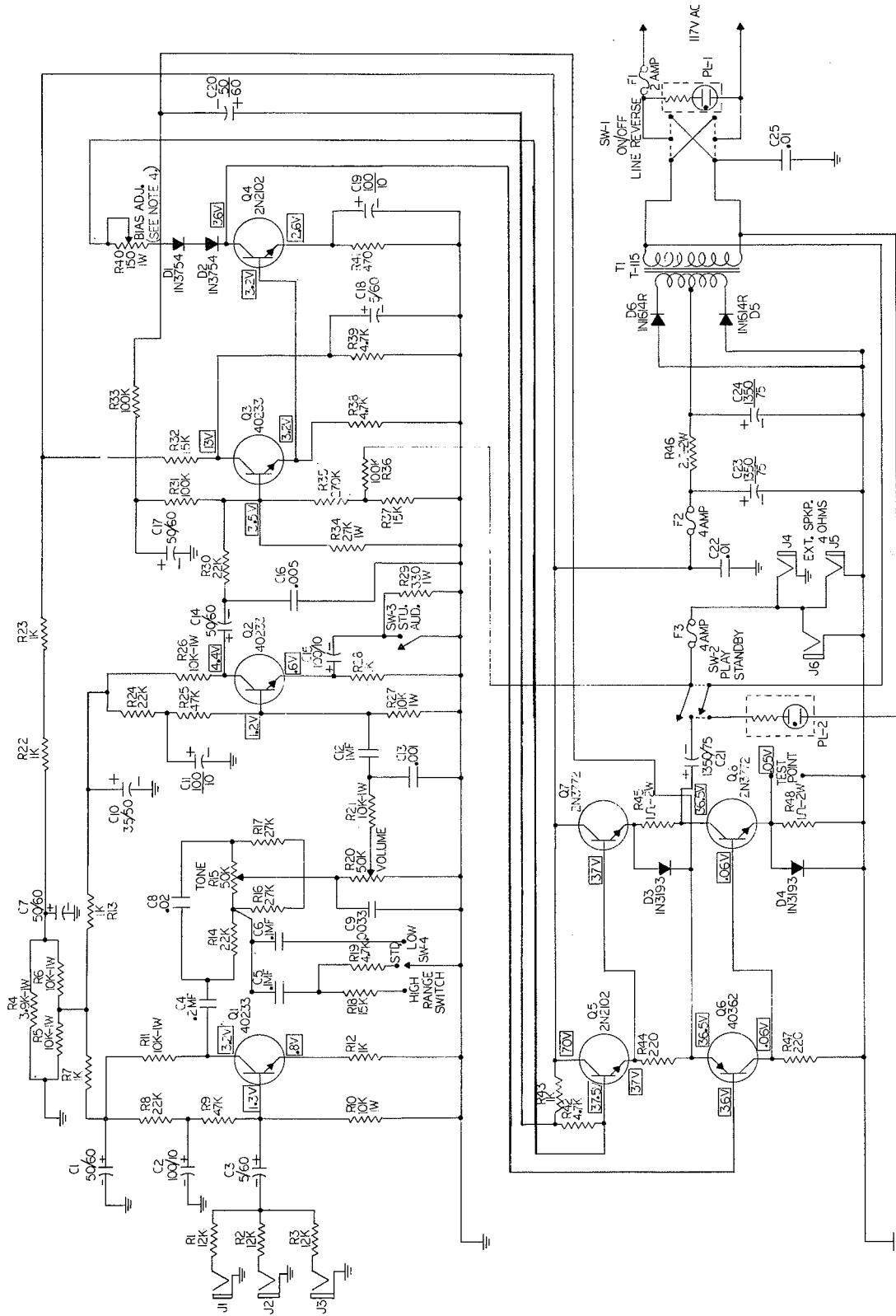
WARDS AIRLINE MODEL GVC-9048A (62-9048) MUSICAL INSTRUMENT AMPLIFIER
