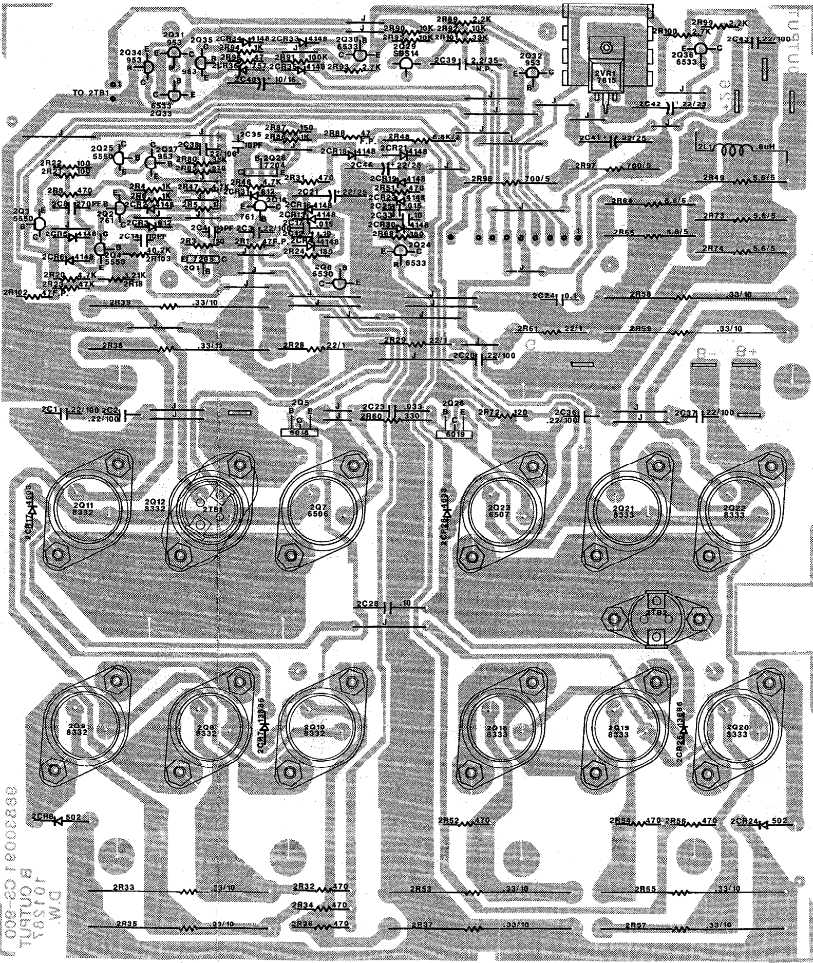
B OUTPUT BD.
