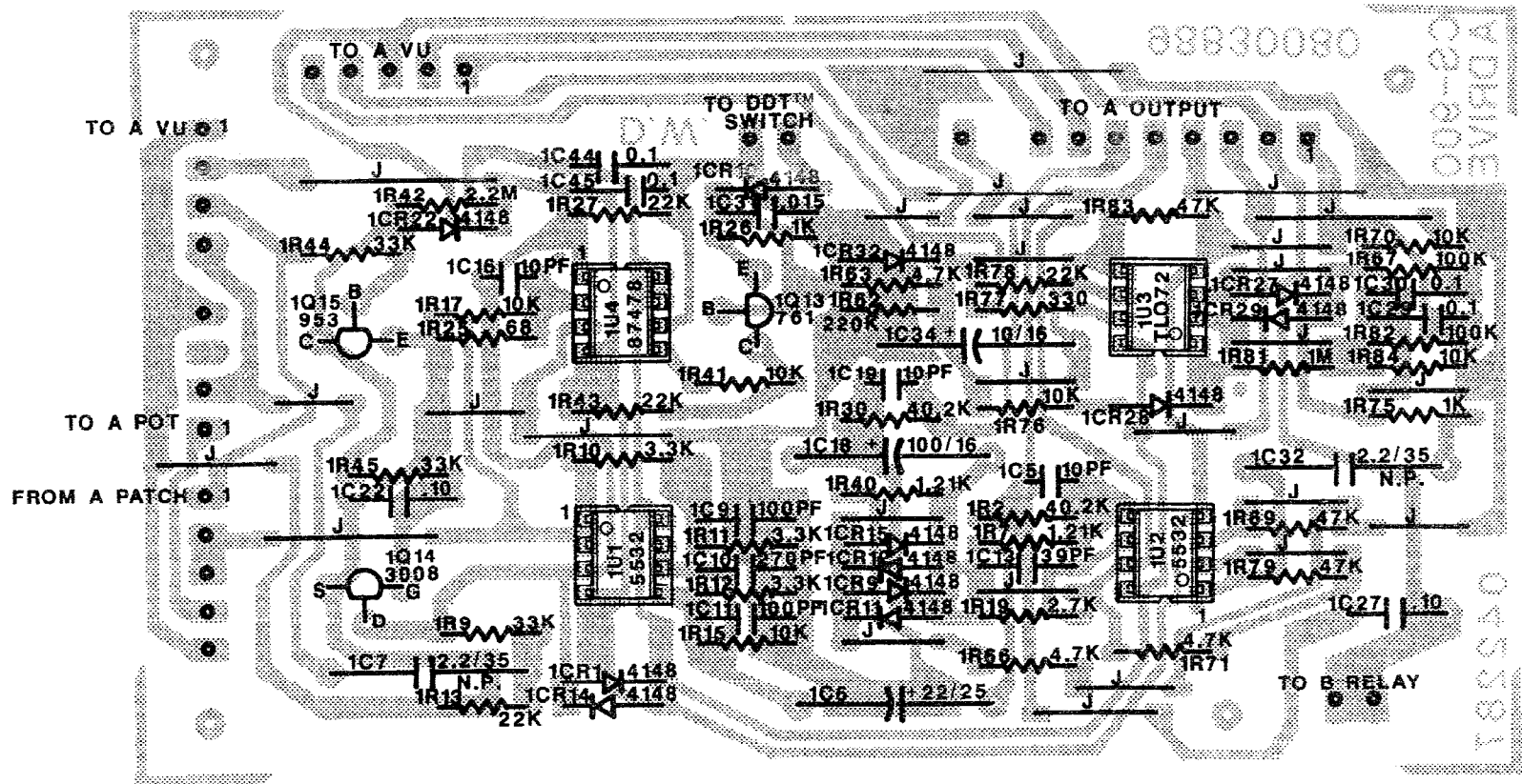
A DRIVE BD.
