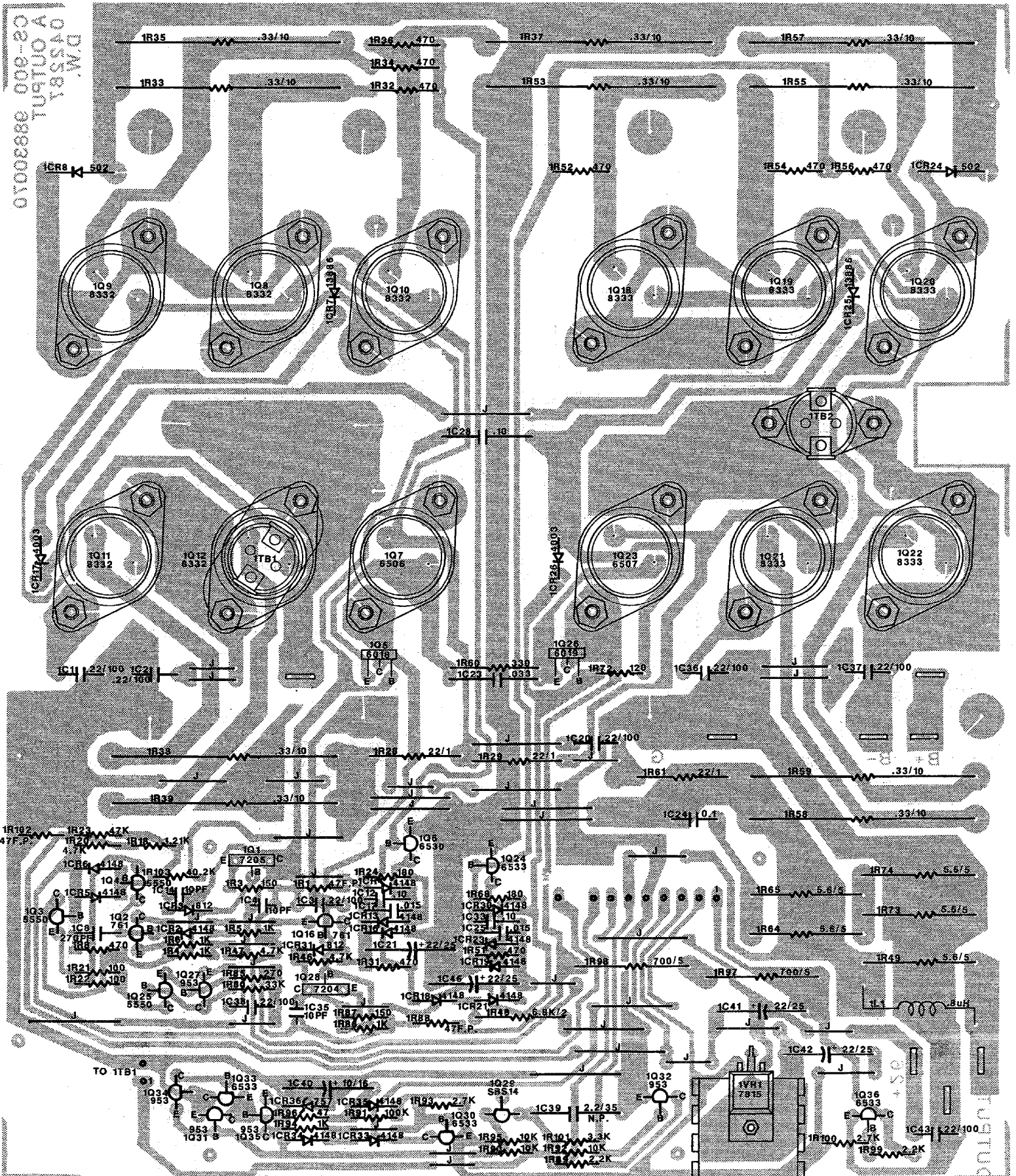
A OUTPUT BD.
