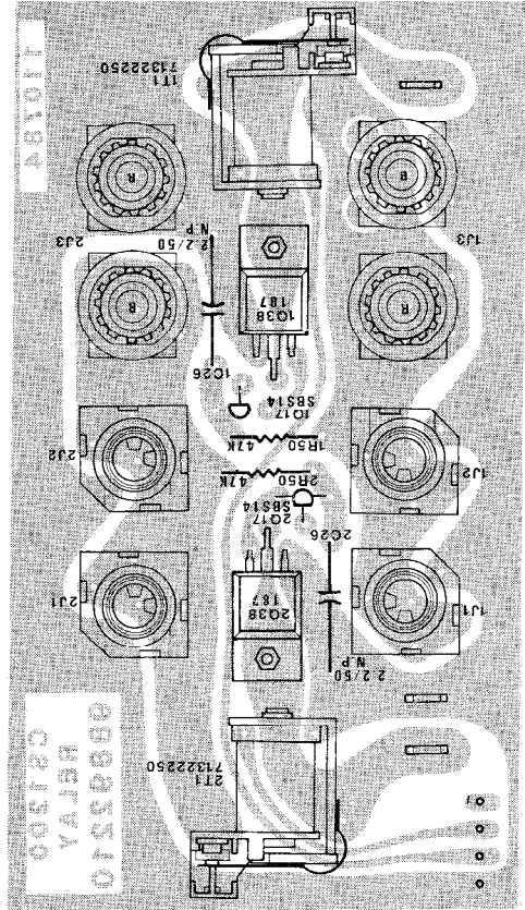
RELAY BD.
