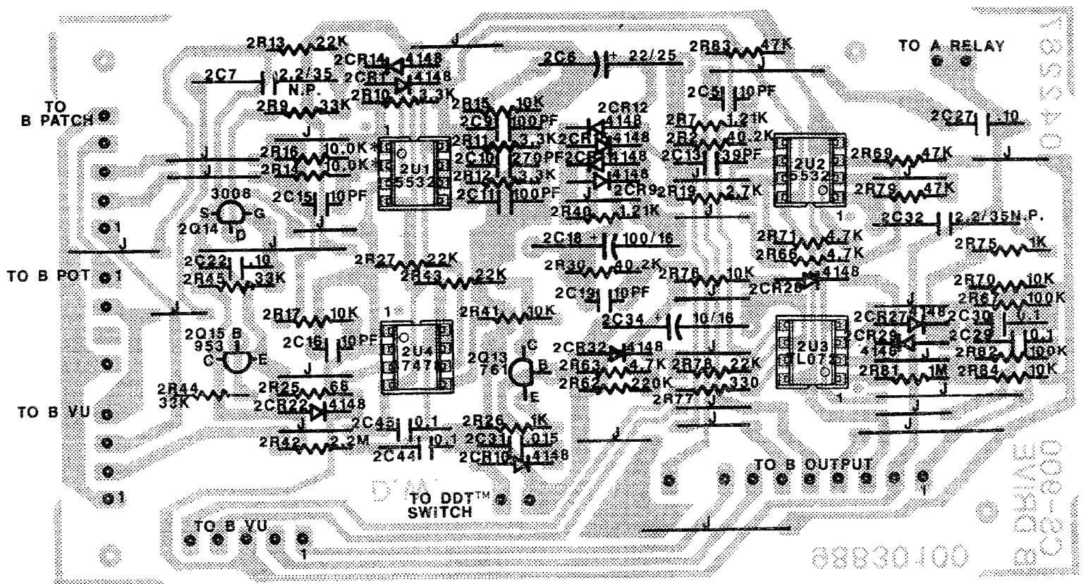
B DRIVE BD.
