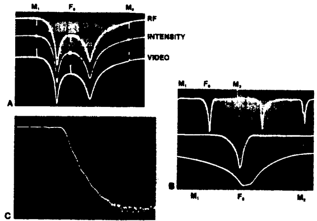
Figure 4. (A) F_0 , M_1 , M_2 markers are displayed as RF, intensity, or video pips. (B) In F_0 - F_2 sweep (top), M_1 and M_2 markers can be used to select limits of M_1 - M_2 sweep (center). The F_0/\Delta F sweep (bottom) with M_1 , M_2 markers sweeps symmetrically about F_0 from 0 to 100% of full band. (C) When used with the 560A Network Analyzer, the 6600A markers can be tilted for optimum display on vertical traces.
