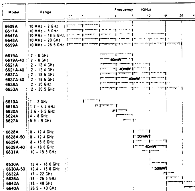
Figure 1. The 6600A Programmable Sweep Generator family covers the 10 MHz to 40 GHz range.
