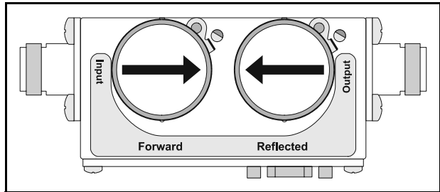
Figure 5 DPS Element Orientation
