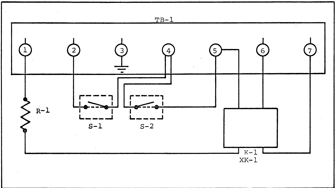
Fig. 4. Schematic Wiring Diagram--Terminal Board Connections and Electrical Components
