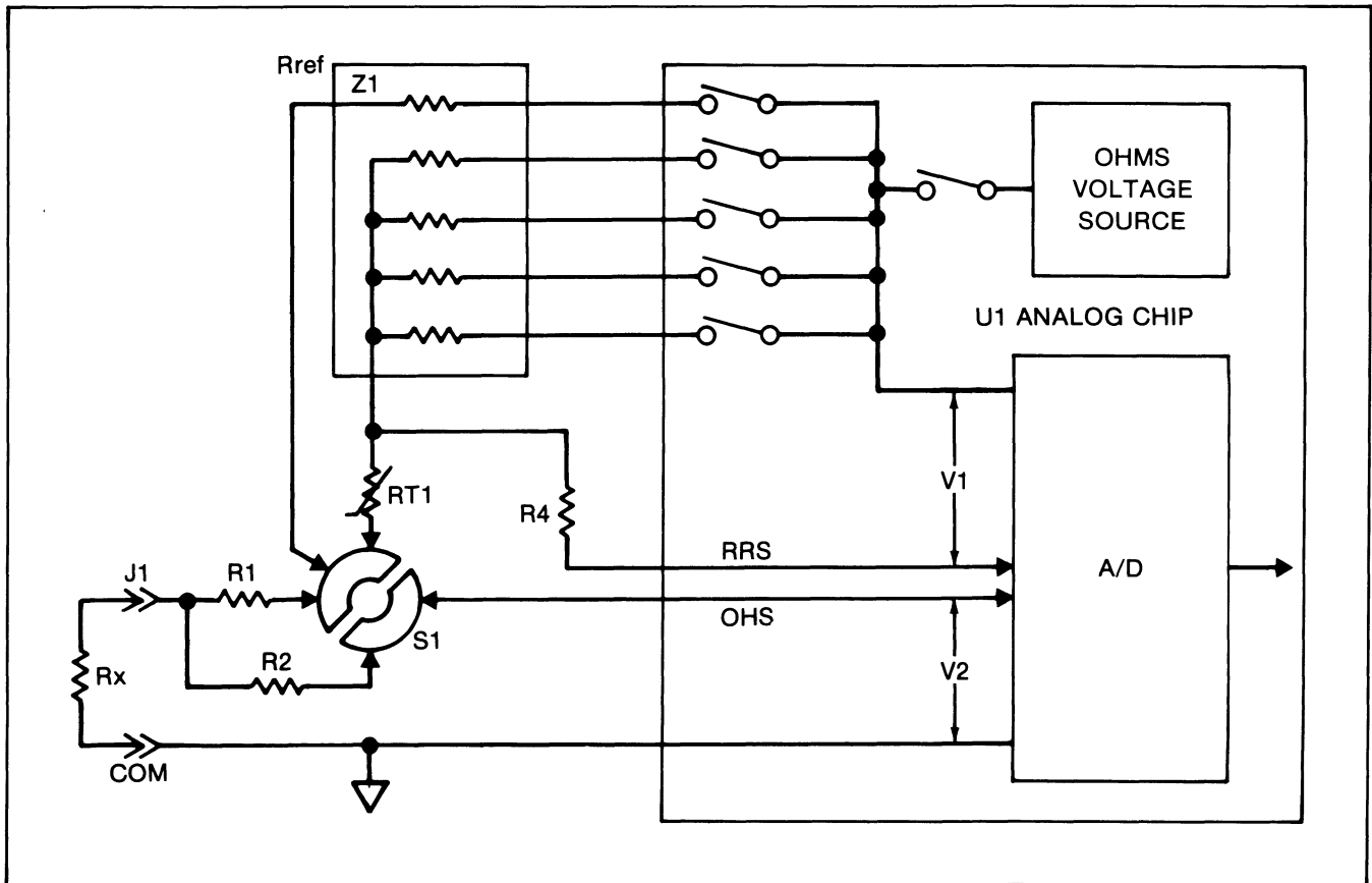
Figure 3-2. Ohms Function
