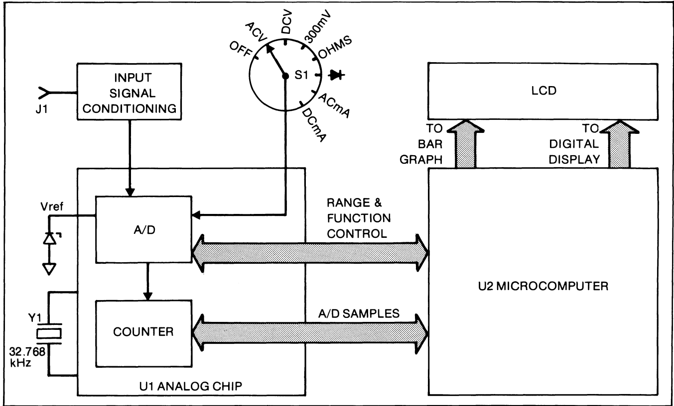
Figure 3-1. Overview
