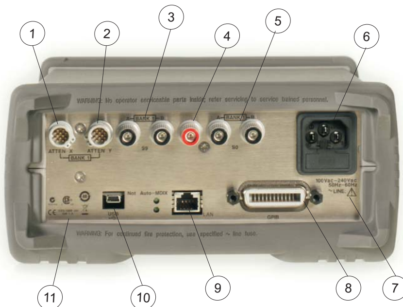
Figure 2 11713B Rear Panel Features
