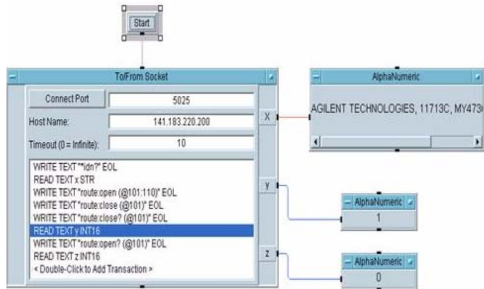
Figure 6-3 Example of control using Agilent VEE
