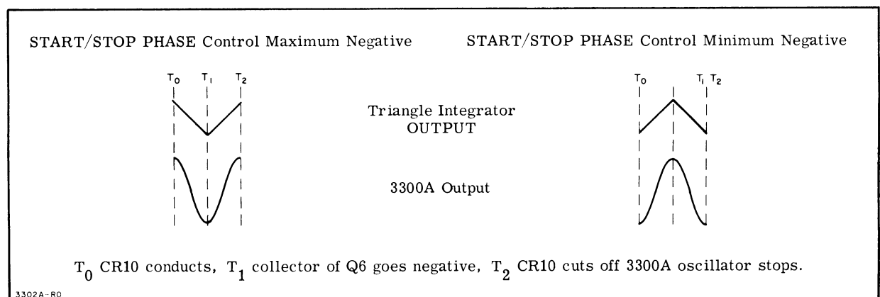
Figure 4-3. Effect of START/STOP PHASE Control on 3300A Triangle Integrator
