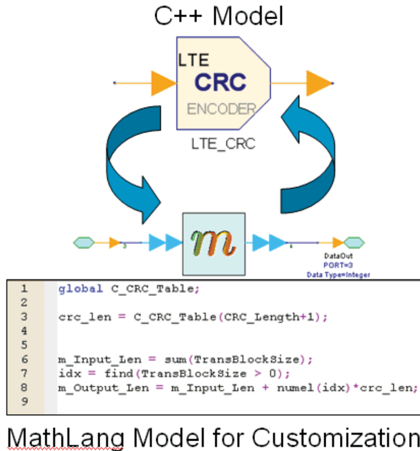
Figure 6. Customization of the SystemVue simulation model.
