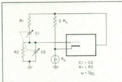
Figure 3. Basic circuit of RC oscillator.
