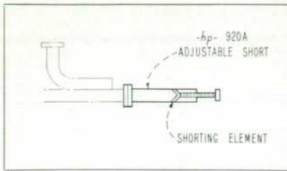
Fig. 10. Model 920A adjustable short connected to output of reflectometer.
