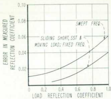
Fig. 4. Accuracy obtained with reflectometer on swept-frequency operation after calibration and on single-frequency operation after minimizing residual signals.
