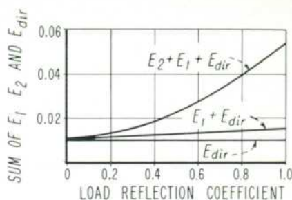
Fig. 9. Sum of three residual signals as a function of load's reflection coefficient.
