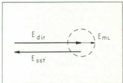
Fig. 12. Reflection E_{srt} from slide-screw tuner cancels directivity signal E_{dir} so that only 0.005 or less reflection from 914A moving load remains.
