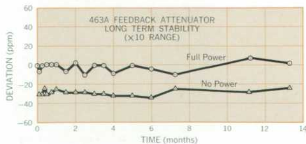
Fig. 3. Long-term stability of the feedback attenuator varies no more than \pm 10 ppm over a period of one year.
