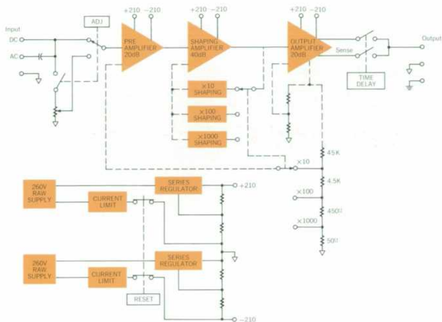
Fig. 2. Fixed gains in the -hp- Model 463A are selected by changing amplifier feedback characteristics by means of a precision feedback attenuator. The attenuator is made up of wire-wound resistors designed for good high-frequency characteristics, low temperature coefficient and good long-term stability.
