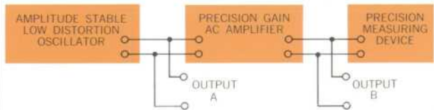
Fig. 5. Generating precision high and low level calibration voltages. In the photo, a digital voltmeter is being used as the precision measuring instrument.
