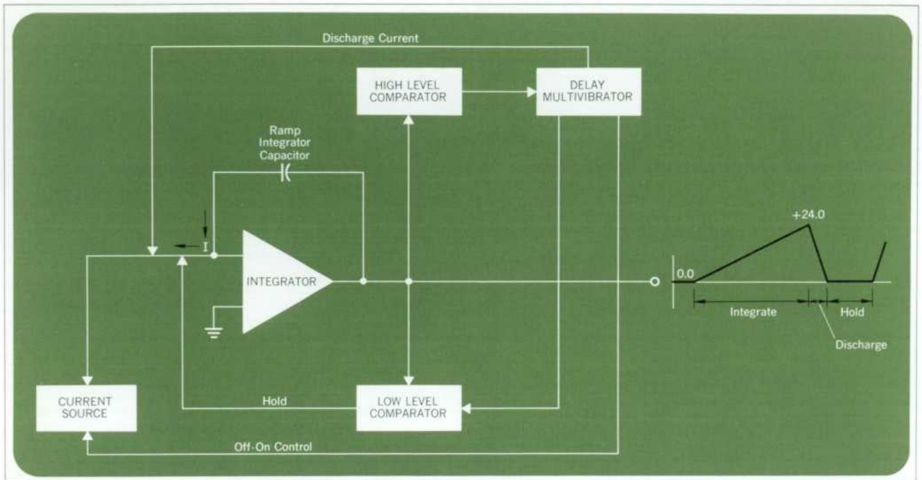
Fig. 3. In this ramp generator circuit of the Model 3305A Plug-In, the sweep time is changed by switching various integrator capacitors and adjusting the current source.
