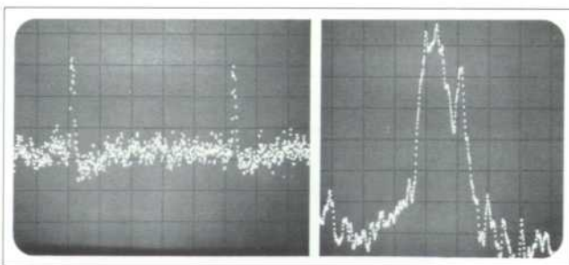
Signal analyzer display of two pulses (left) averaged for 32 sweeps. These pulses are buried in noise in the raw input signal to the averager and are barely discernible. Their spacing serves to identify this source, known as CP1919. An expanded view (right) shows its characteristic shape.
