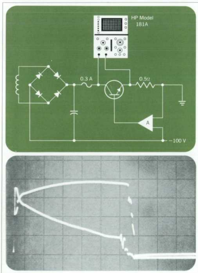
Fig. 4. To examine current and voltage in the series regulator when the output is shorted, the scope is connected as in the schematic. Current and voltage curves (transients) are as shown. Instantaneous power can be plotted by multiplying current and voltage for a number of difference instants in time.
