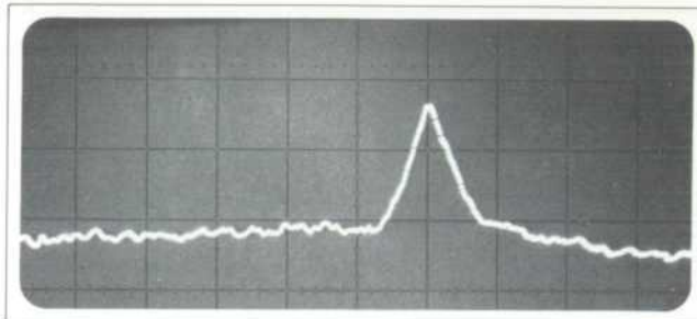
Characteristic shape of a pulsar waveform. This is CP0950, the strongest of the originally published pulsars.
