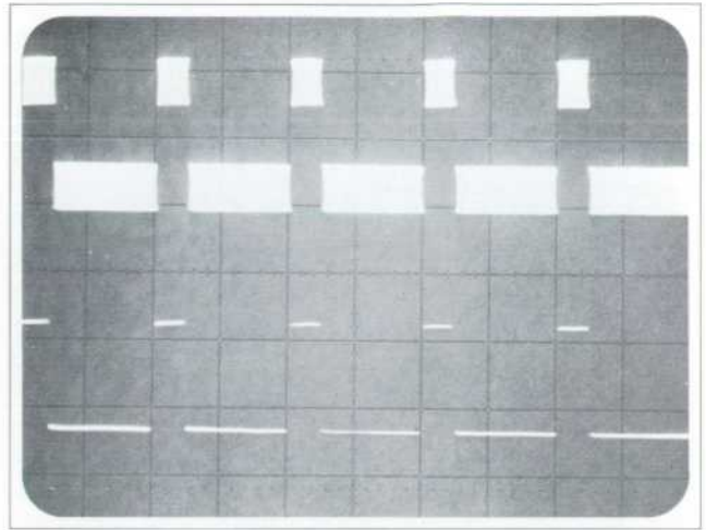
Fig. 5. The top trace demonstrates a thick trace produced when a 60 Hz signal is superimposed on the pulse train. The bottom trace shows a single-shot presentation which eliminates the effect of the 60 Hz interference.
