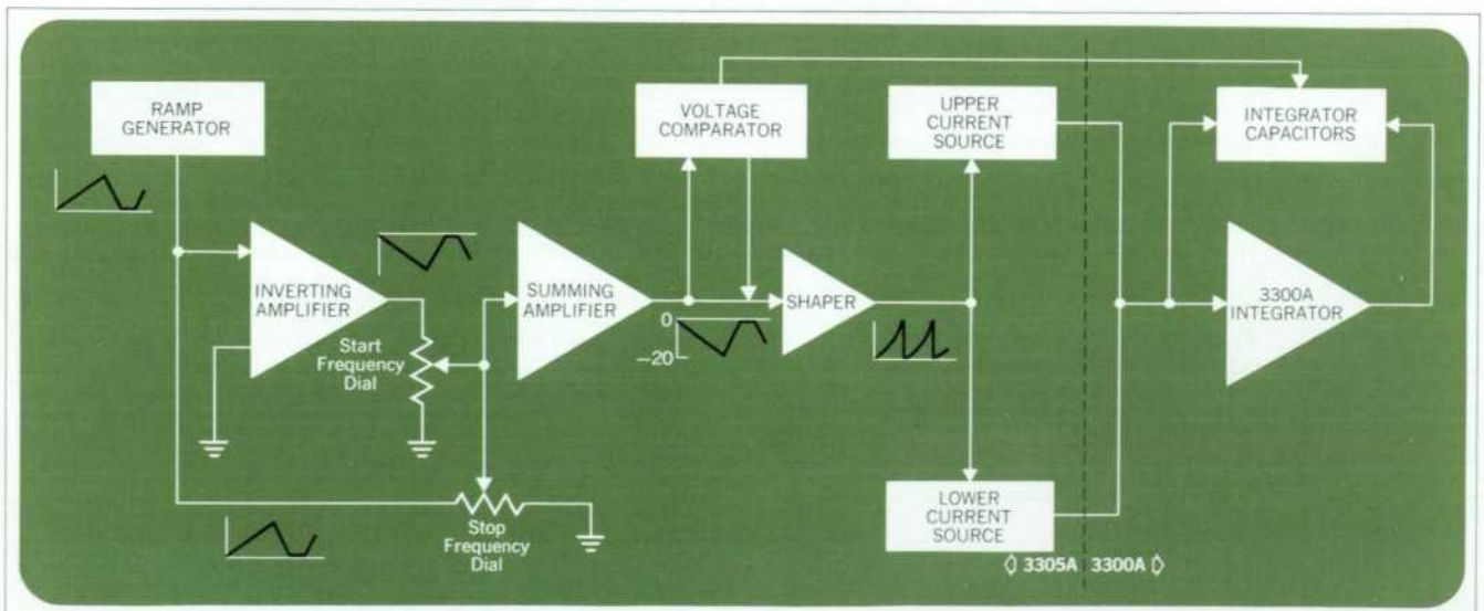
Fig. 4. Upper and lower current sources in the Model 3305A are designed with more precise control of currents to allow four decades of sweep. The sweep mode selection is effected by switching within the ramp generator.
