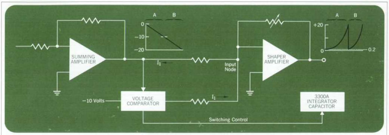
Fig. 6. The two exponential curves at the right are generated from the single ramp at the left. As the ramp voltage goes from 0 to -10 , current is drawn from the shaper amplifier causing its output to rise exponentially from 0.2 to 20 volts. At -10 volts on the ramp, the voltage comparator switches the precise amount of current being drawn. This causes the shaper amplifier to reset to 0.2 volt. The voltage comparator continues to supply current as the ramp proceeds from -10 to -20 volts, resulting in the second exponential B, at the right.
