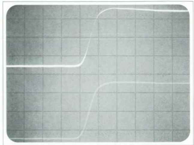
Fig. 2. Double exposure photo of a fast rise time, low repetition rate pulse. The lower trace was exposed for 10 seconds with conventional scope operation. The upper trace was exposed for 1 second after letting the trace integrate up for 10 seconds in the variable persistence mode.
