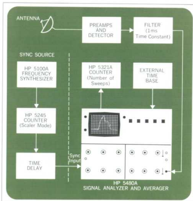
In the system for viewing the pulsar signals, the time delay is used so that the pulses may be shifted on the CRT screen. An external time base was used to obtain two periods across the CRT.
