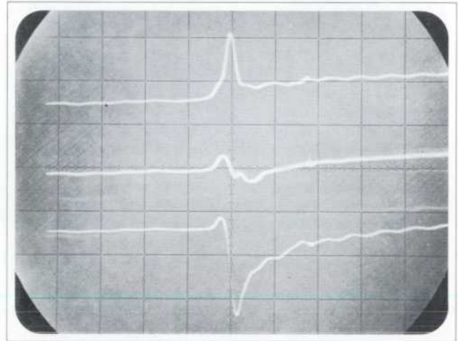
Fig. 6. Comparison of three 50-ohm terminations using a variable persistence scope and the HP Model 1415A Time Domain Reflectometer. The top trace shows an inductive spike at the termination, the bottom trace shows a capacitive spike and the middle trace is compensated termination. These traces were stored for comparison for about one hour.
