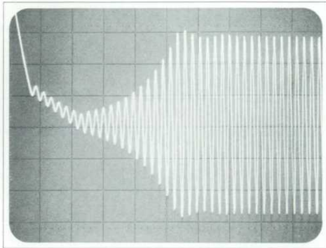
Fig. 3. A fast, easy way to determine how long it takes for an oscillator to stabilize. Here it takes the oscillator about 4 seconds to rise to its peak-to-peak value. This type of measurement is important in determining the measurement speed of a system.
