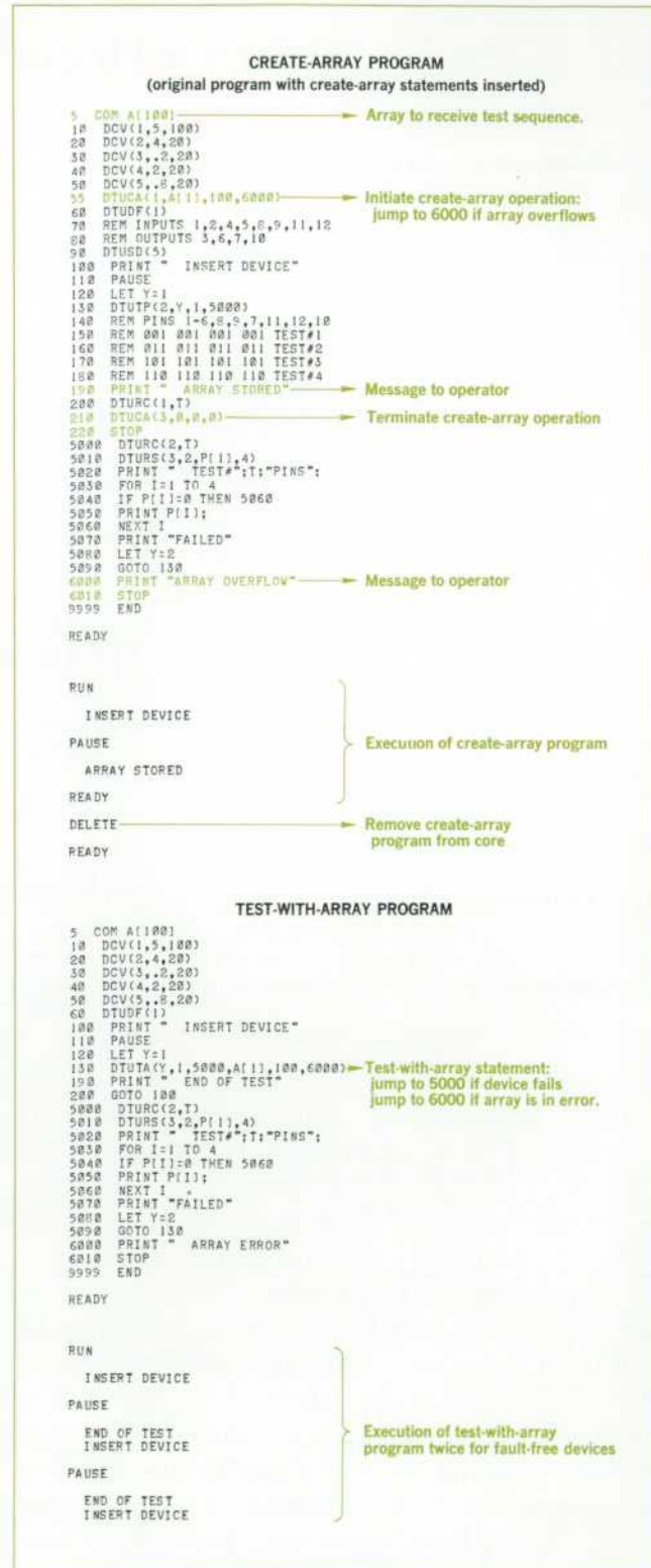
Fig. 4. Test pattern created and checked out in interactive mode is stored in compiled form by inserting 'create array' statements in program. Tests run much faster in compiled mode: for a 12-pin device maximum test rates are approximately 22,000 tests per second in compiled mode and 150 in interactive mode.
