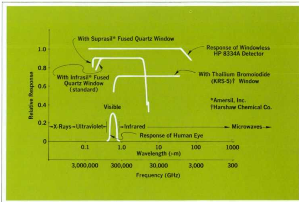
Fig. 4. Flat response of detector allows accurate broadband measurements. Spectral range varies with transmission characteristics of window mounted in front of thermopile.
