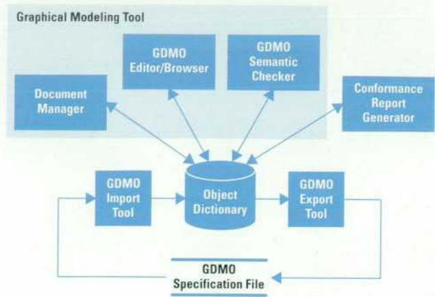
Fig. 2. The GDMO modeling toolset.
