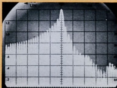
Same conditions as at left except 1 MHz/Div spectrum width
