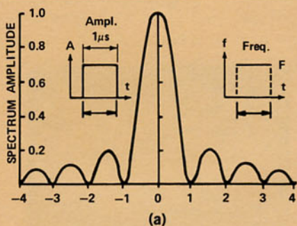
(a) Spectrum of rectangular pulse without AM or FM occurring during pulse. Shape is that of \frac{\sin \omega \frac{T}{2}}{\omega \frac{T}{2}} function.
