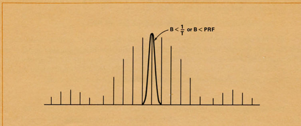
Figure 6. IF bandwidths smaller than PRF.
