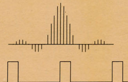
Figure 4b. Wider pulse than 4a causes narrower lobes, but line density remains constant since PRF is unchanged.
