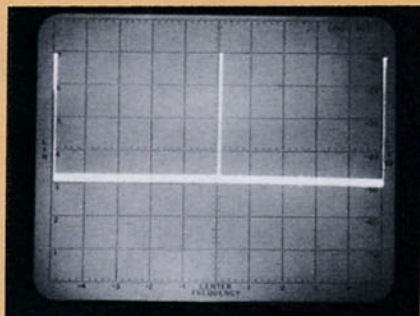
Figure 20. Same signal, but B = 300 kHz and scan time 2 ms/Div. The PRF can be measured to 1/10 ms = 100 Hz.
