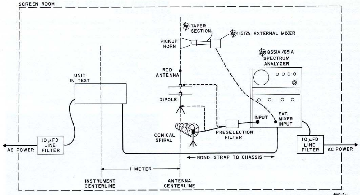
Figure 24. Suggested setup for measuring radiated RFI with the Spectrum Analyzer and appropriate antennas.
