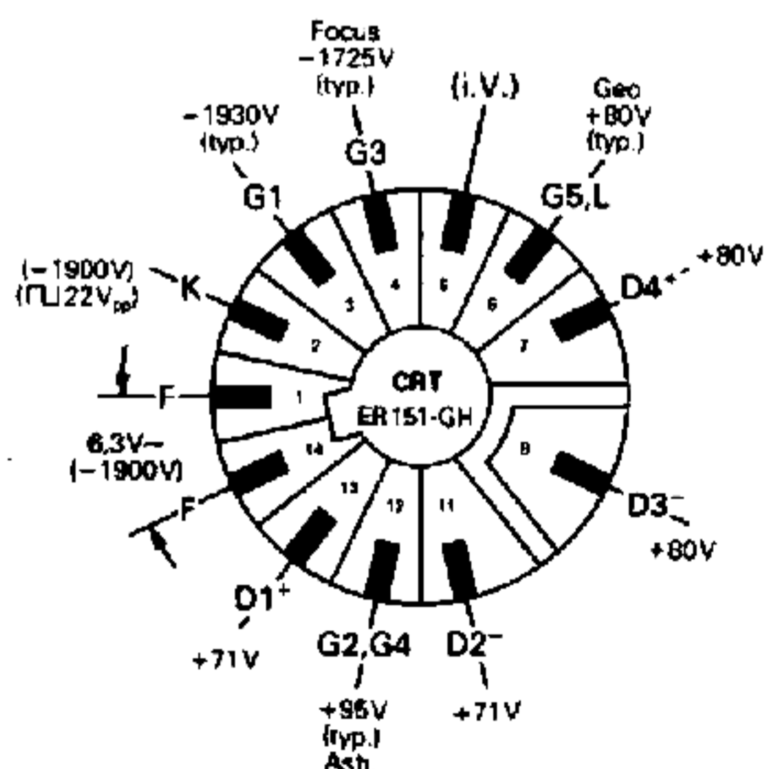
Voltages at the CRT socket
