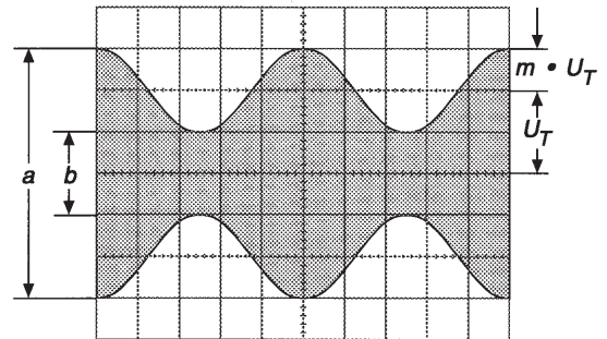
Figure 2 Amplitude modulated oscillation: F = 1 MHz; f = 1 kHz; m = 50 %; U_T = 28.3 \text{ mV}_{\text{rms}} .
