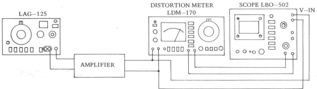
Fig. 2-2 Harmonic distortion measurement.
