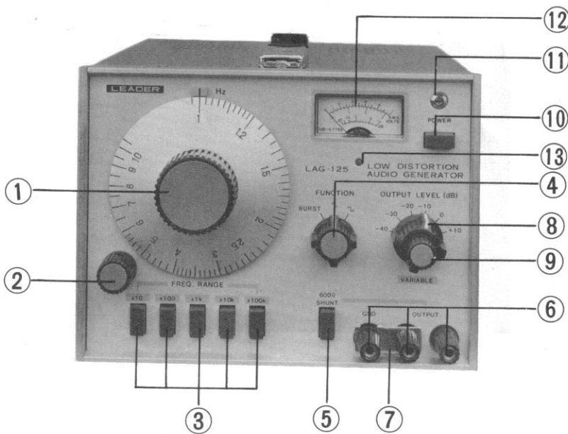
Fig. 1-1 Front panel.
