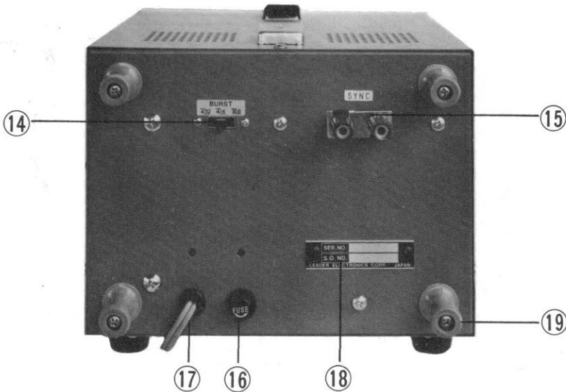
Fig. 1-2 Rear panel functions.
