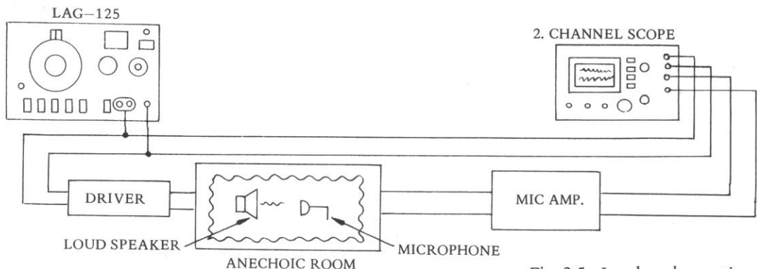
Fig. 2-5 Loudspeaker testing.
