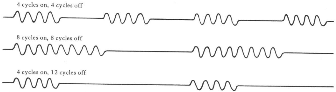
Fig. 2-4 Burst signals.
