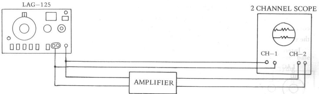
Fig. 2-6 Amplifier testing with burst signals.
