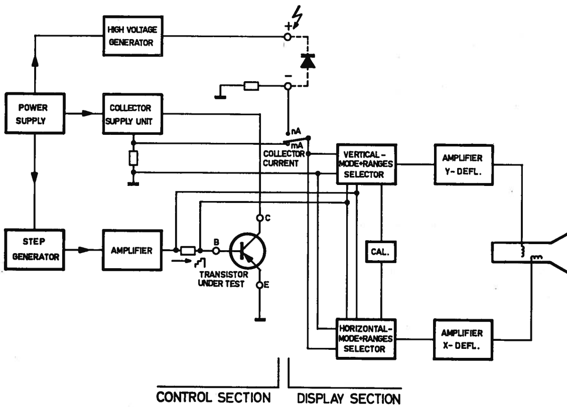
Fig. 1. Basic construction
