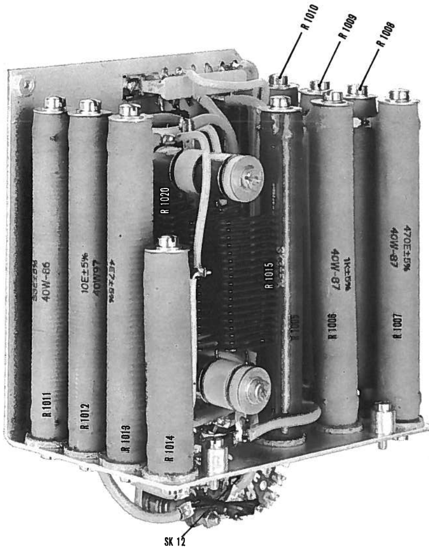
Fig. 74. Collector-load unit U10, taken off
