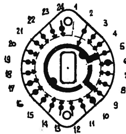
Fig. 91. Switch wafers SK12
