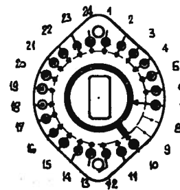
Fig. 92. Switch wafers SK13
