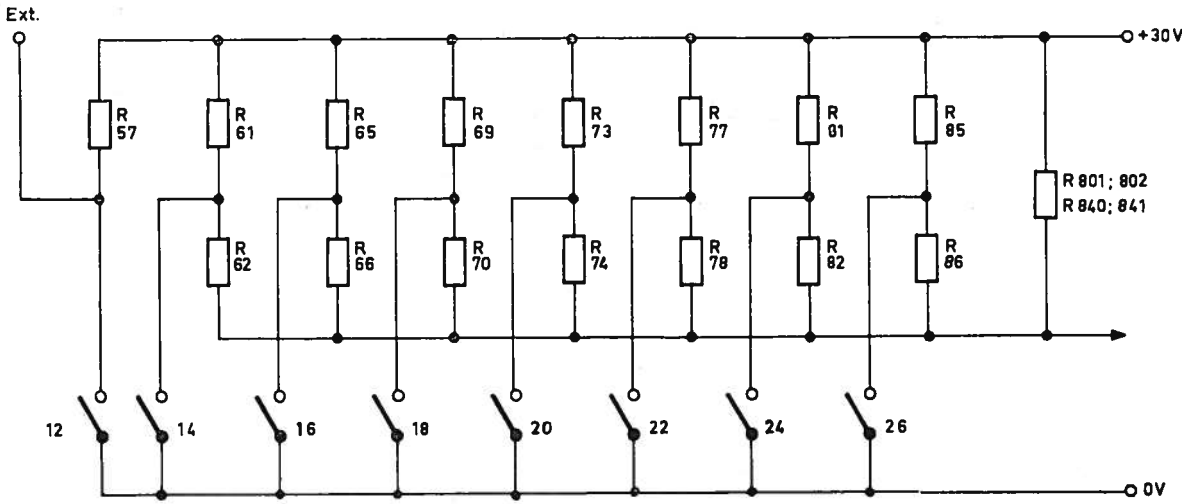
Fig. 53. Principle of the ring counter
