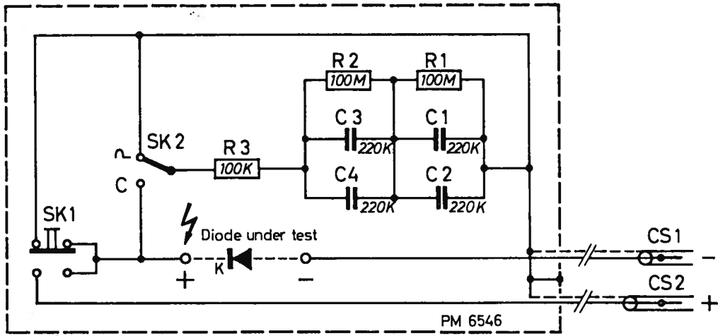
Fig. 87. Diagram PM 6546
