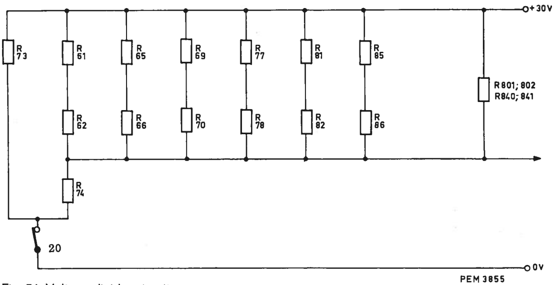
Fig. 54. Voltage-divider circuit
