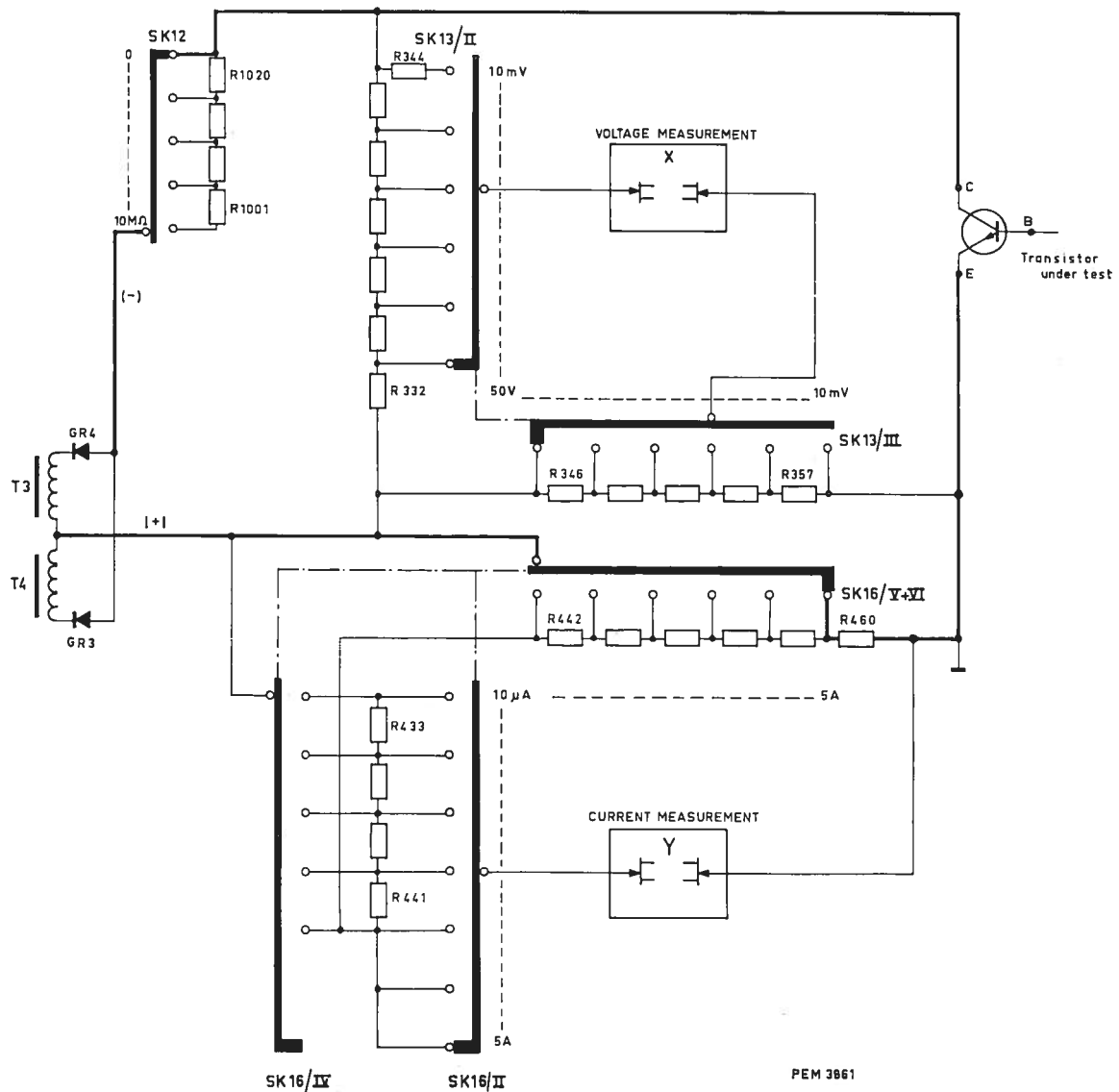
Fig. 58. Collector-current circuit
