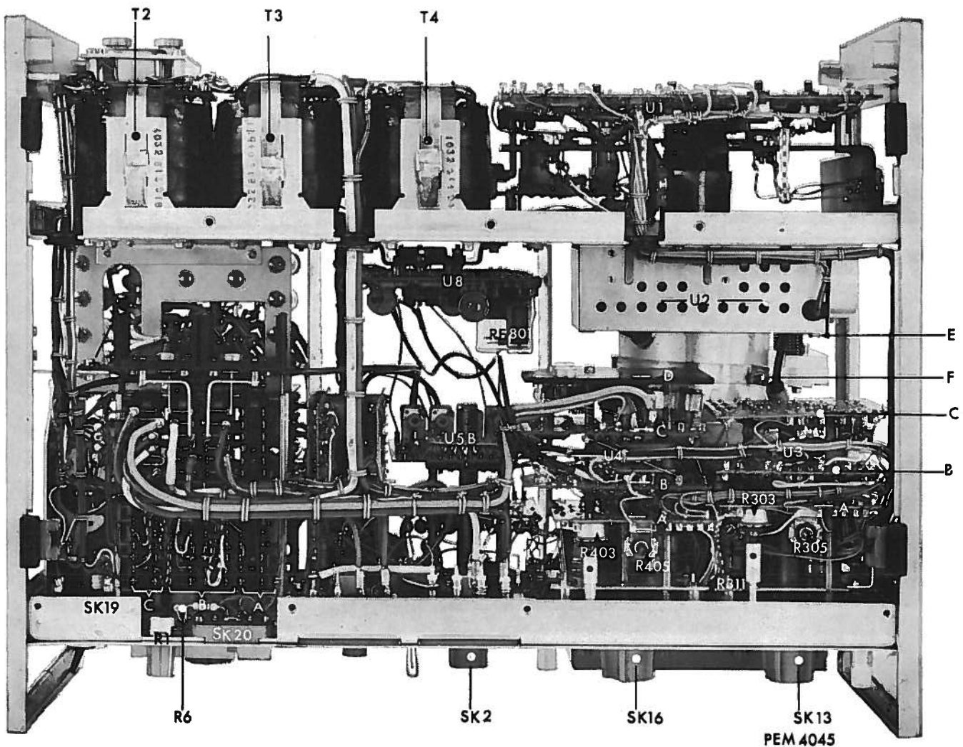
Fig. 64. Bottom view
