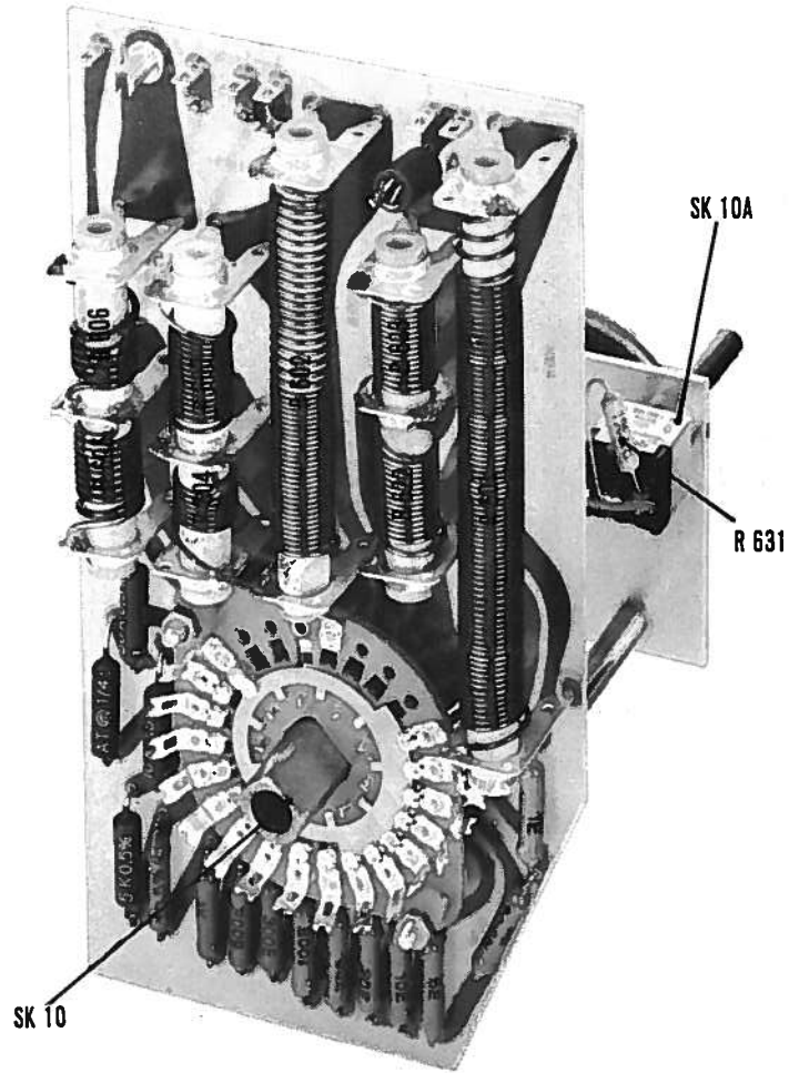
Fig. 69. Shunt unit U6, taken off
