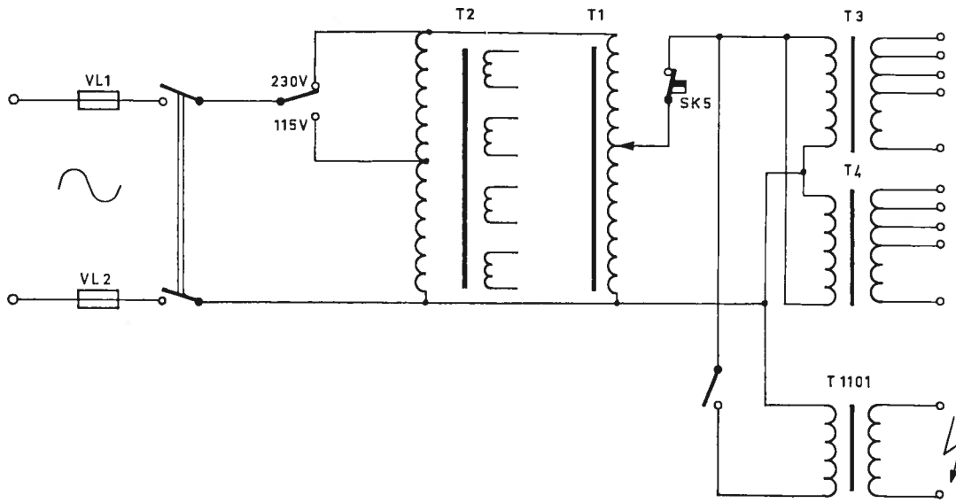
Fig. 48. Supply part
