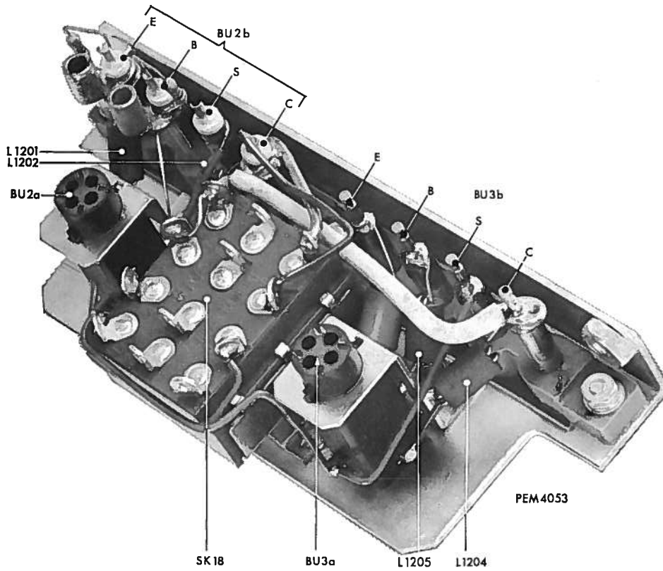
Fig. 76. Socket unit U12, taken off
