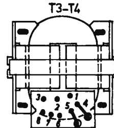
Fig. 95. Connection diagram for collector transformers T3 and T4
