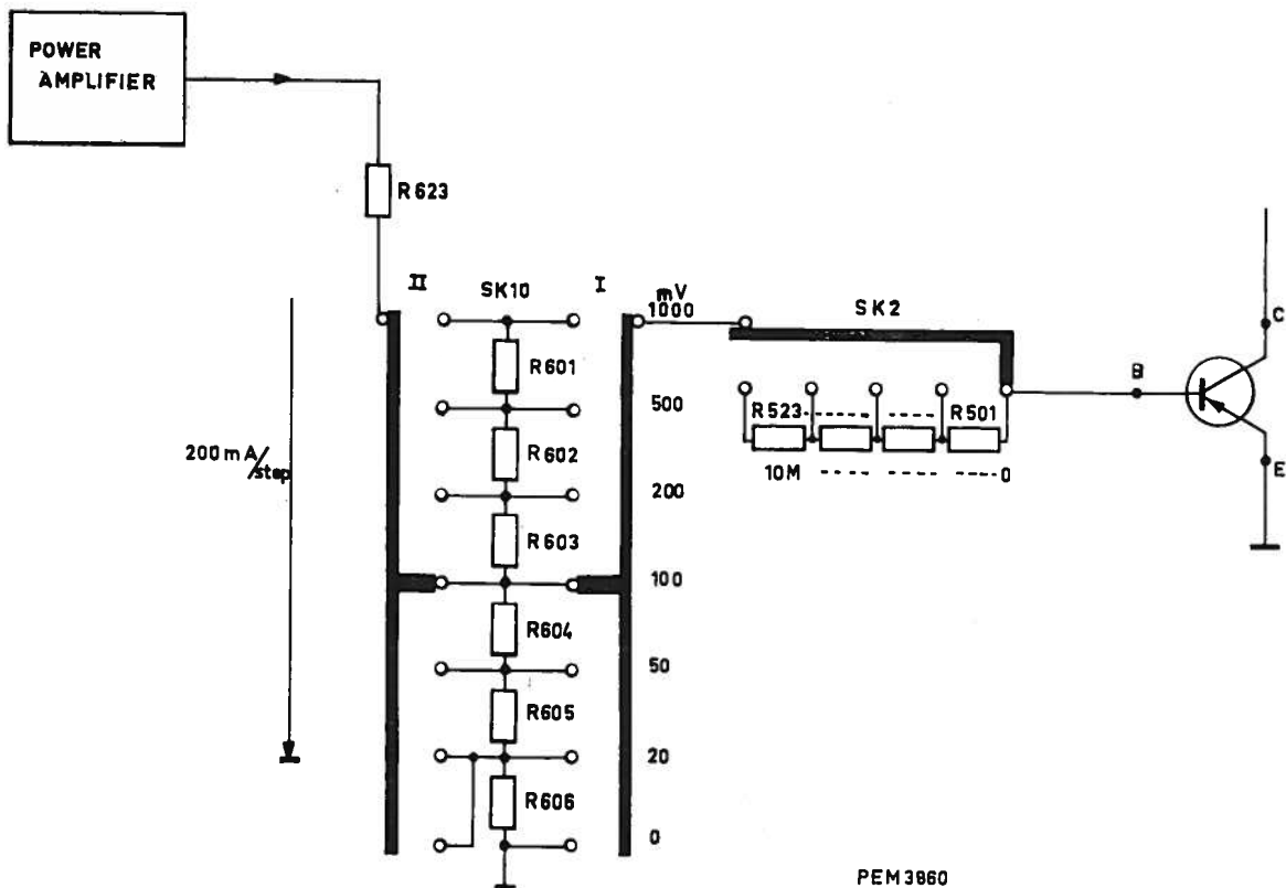
Fig. 57. Voltage drive
