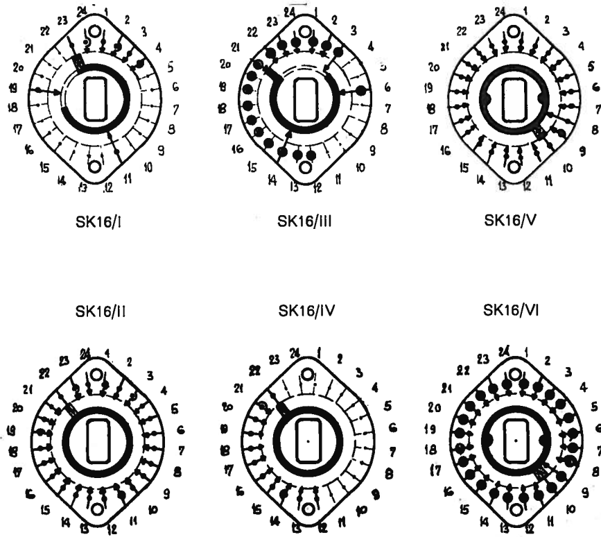
Fig. 93. Switch wafers SK16
