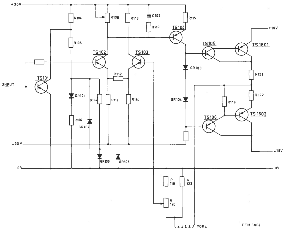
Fig. 61. X-Power amplifier
