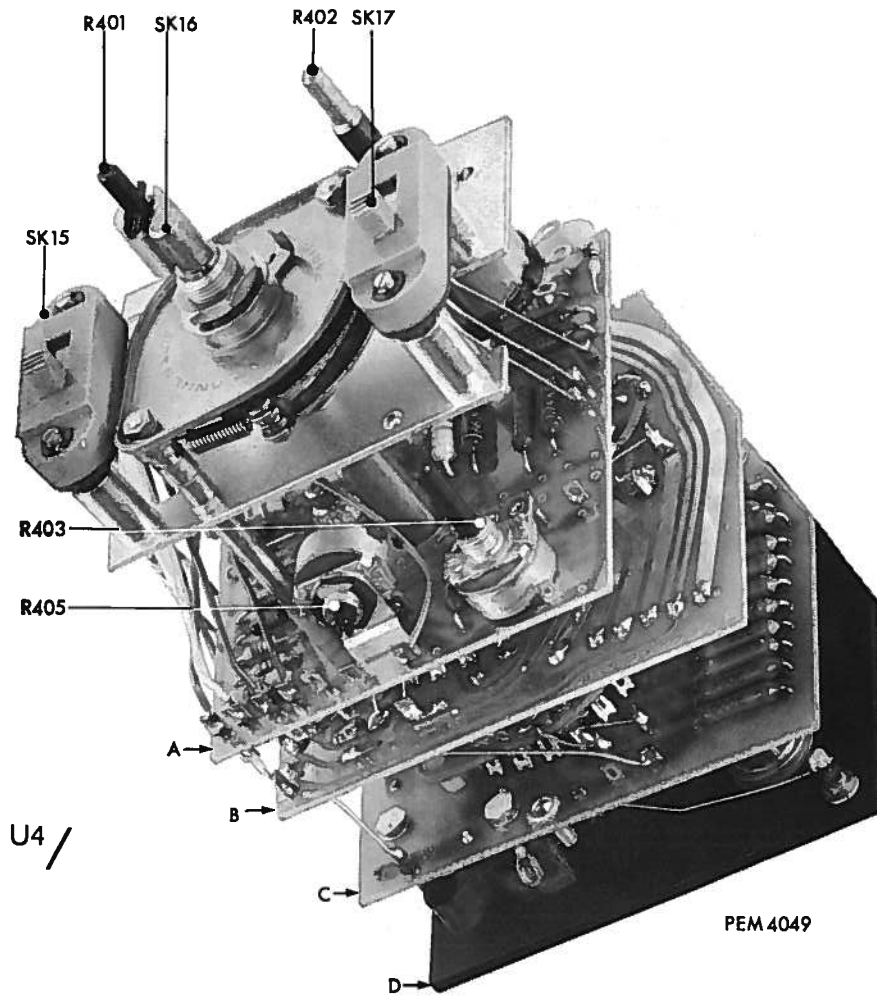
Fig. 67. Y-Deflection unit U4, taken off
