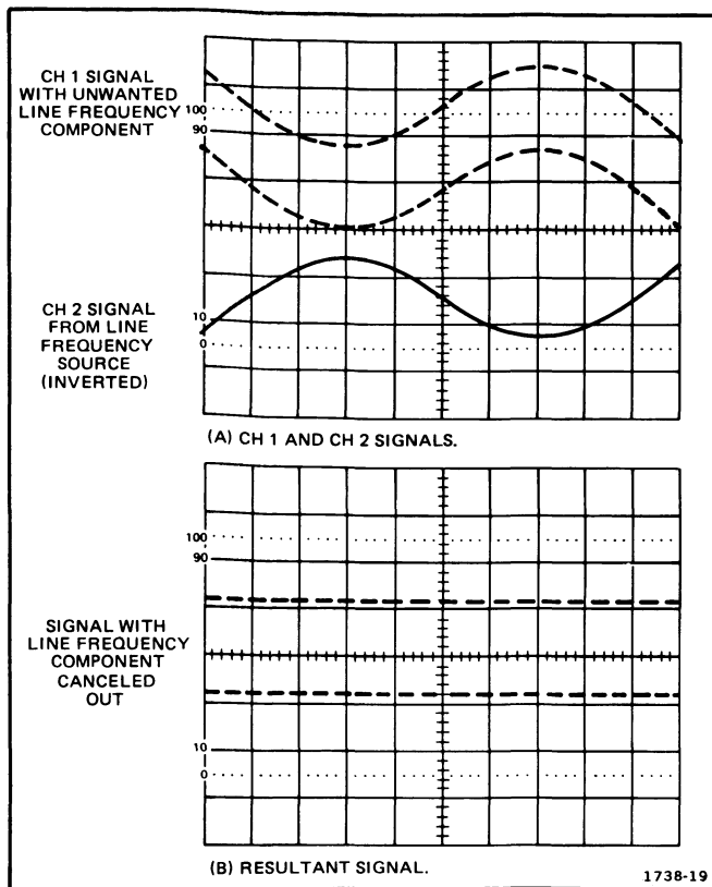
Fig. 17. Common-mode rejection.
