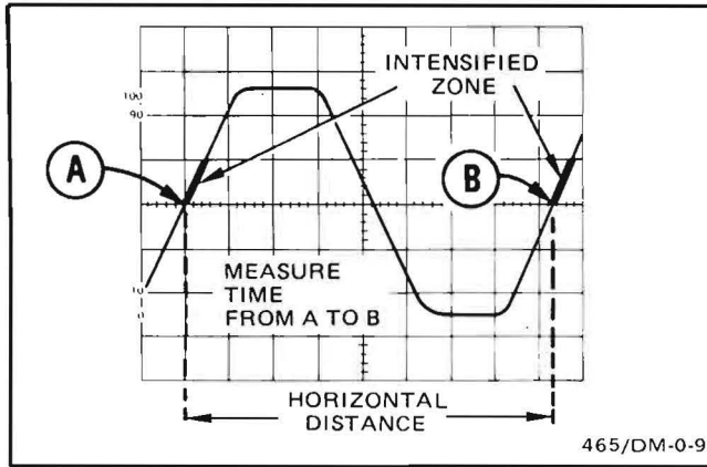
Fig. 26. Time duration.
