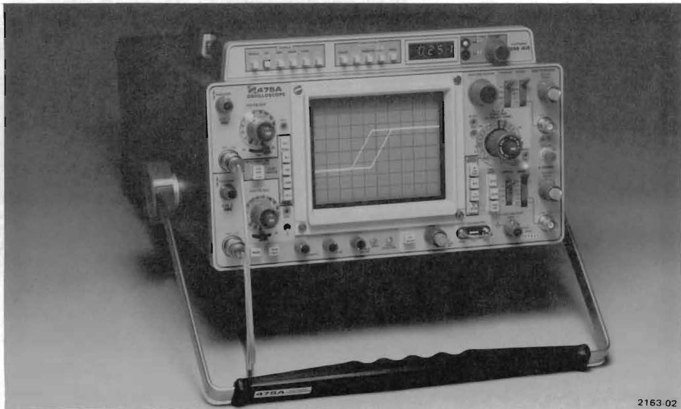
475A Oscilloscope with DM44 Digital Multimeter.
