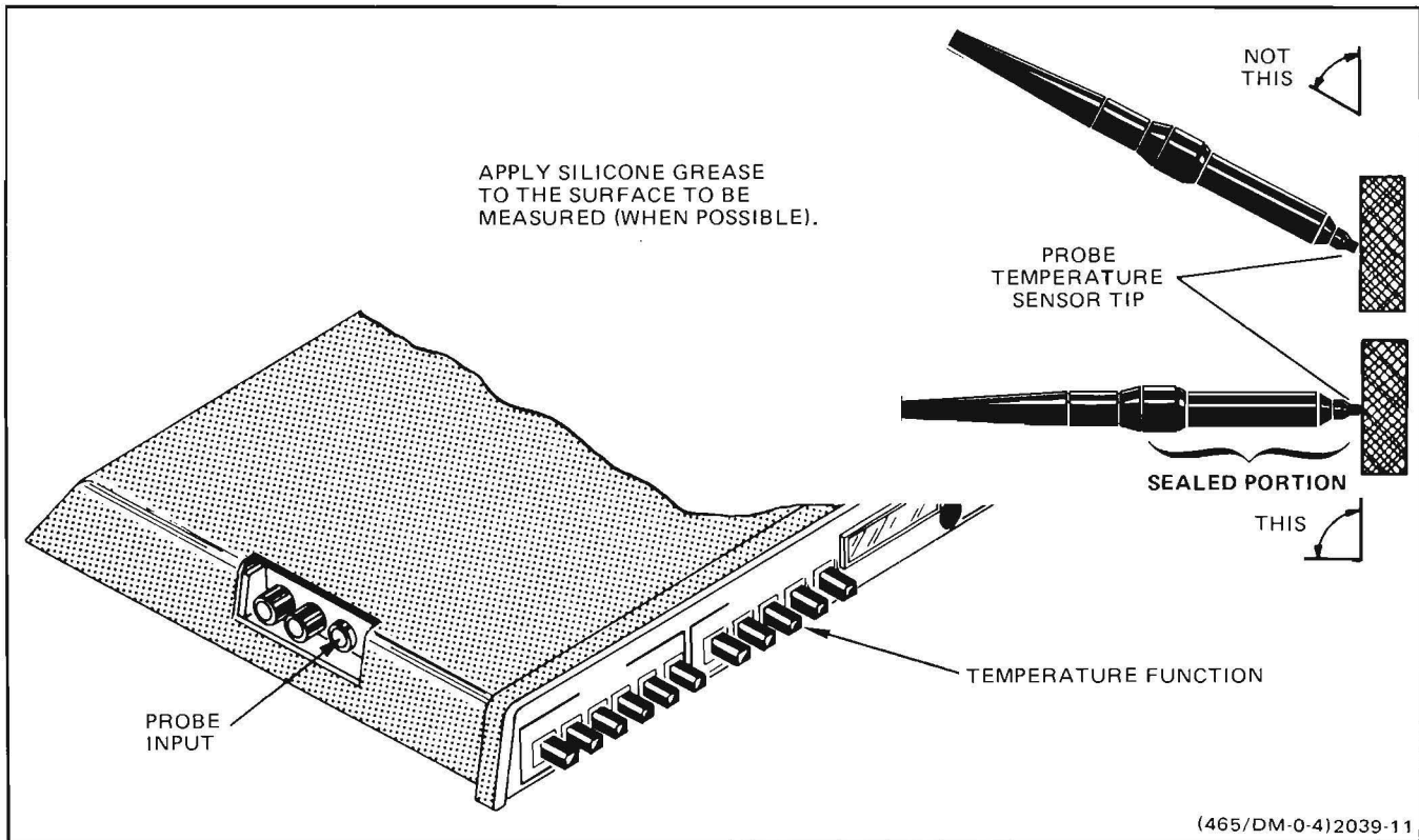
Fig. 10. Temperature.
