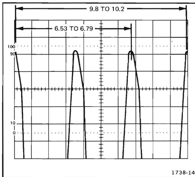
Fig. 12. Basic 475A timing check.
