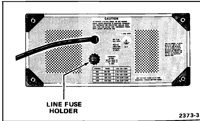
Fig. 3. Line fuse location on Rear Panel.
