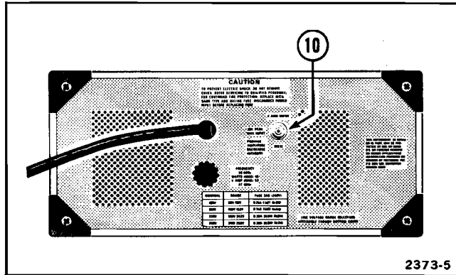
Fig. 5. External Z-AXIS INPUT on Rear Panel.
