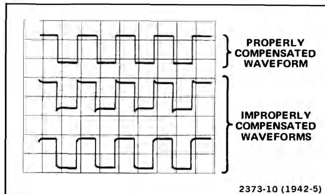
Fig. 10. Probe compensation.
