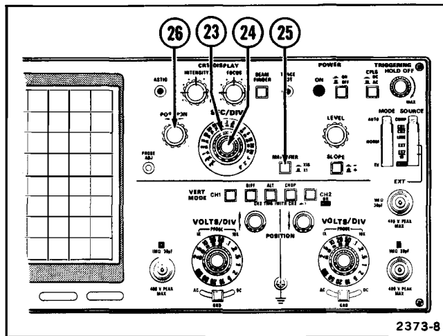
Fig. 8. Horizontal system controls.
