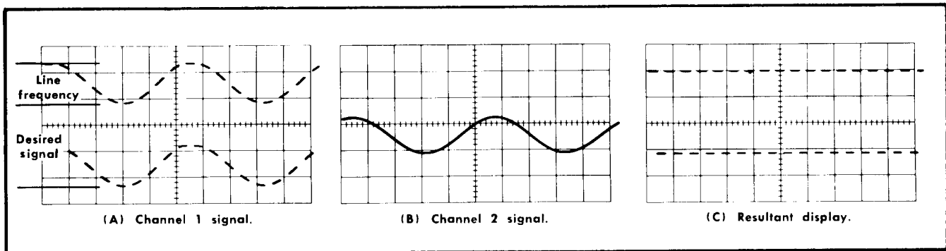
Fig. 2-28. Using the ADD feature for common-mode rejection. (A) Channel 1 signal contains desired information along with line-frequency component, (B) Channel 2 signal contains line-frequency only, (C) CRT display using common-mode rejection.
