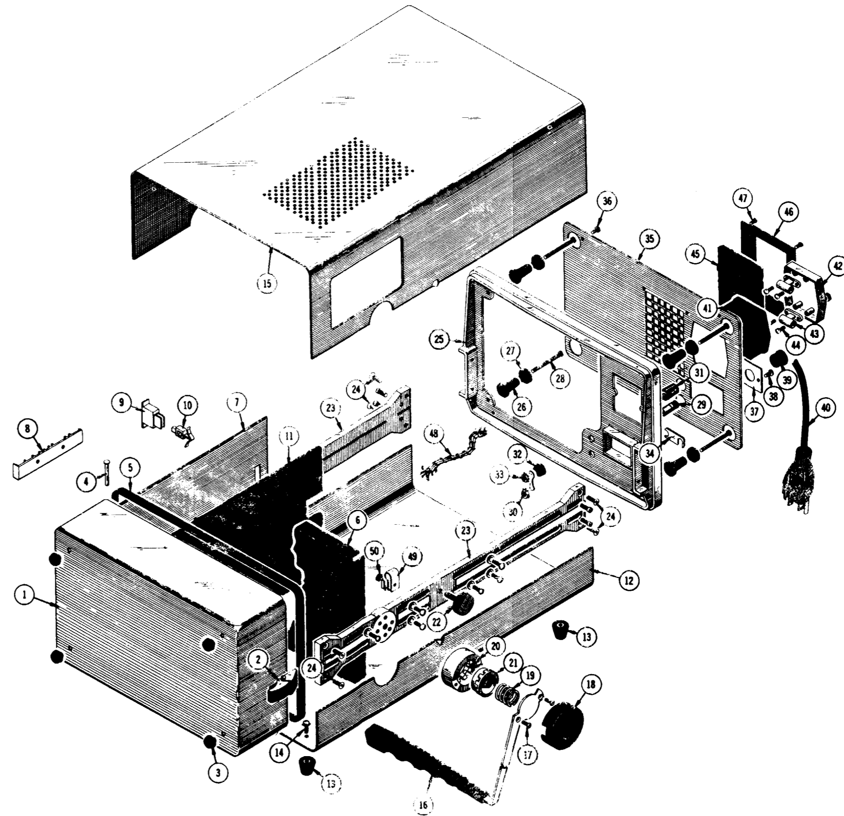
FIG. FO-7 FRAME & CABINET
