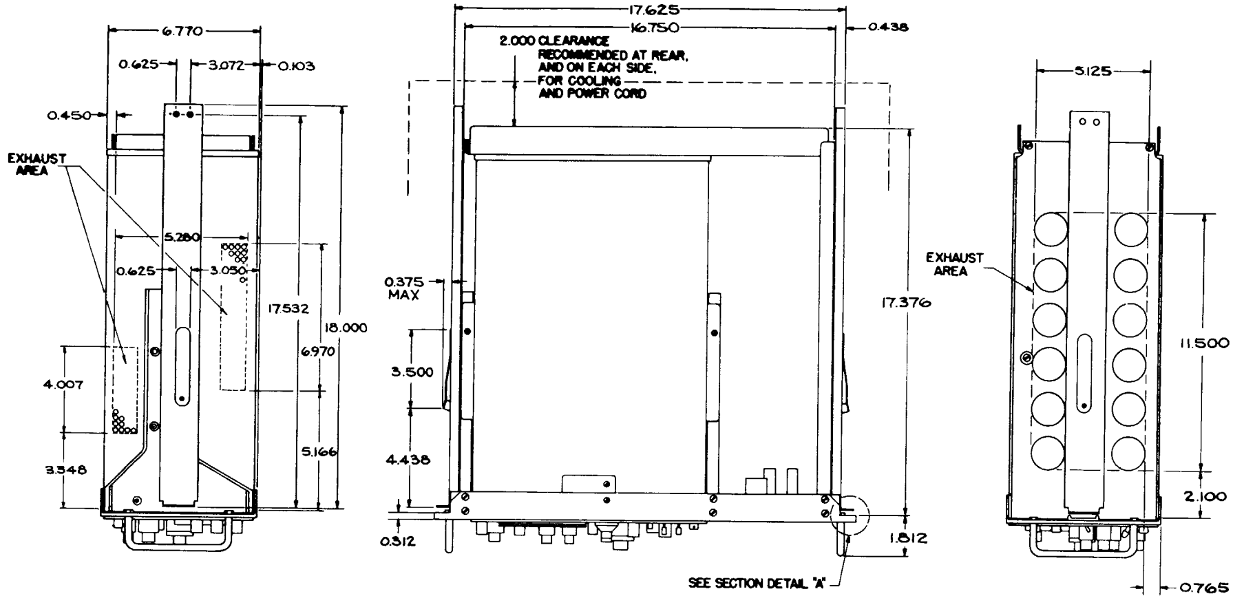
FIGURE 10-14. DIMENSIONAL DRAWING
