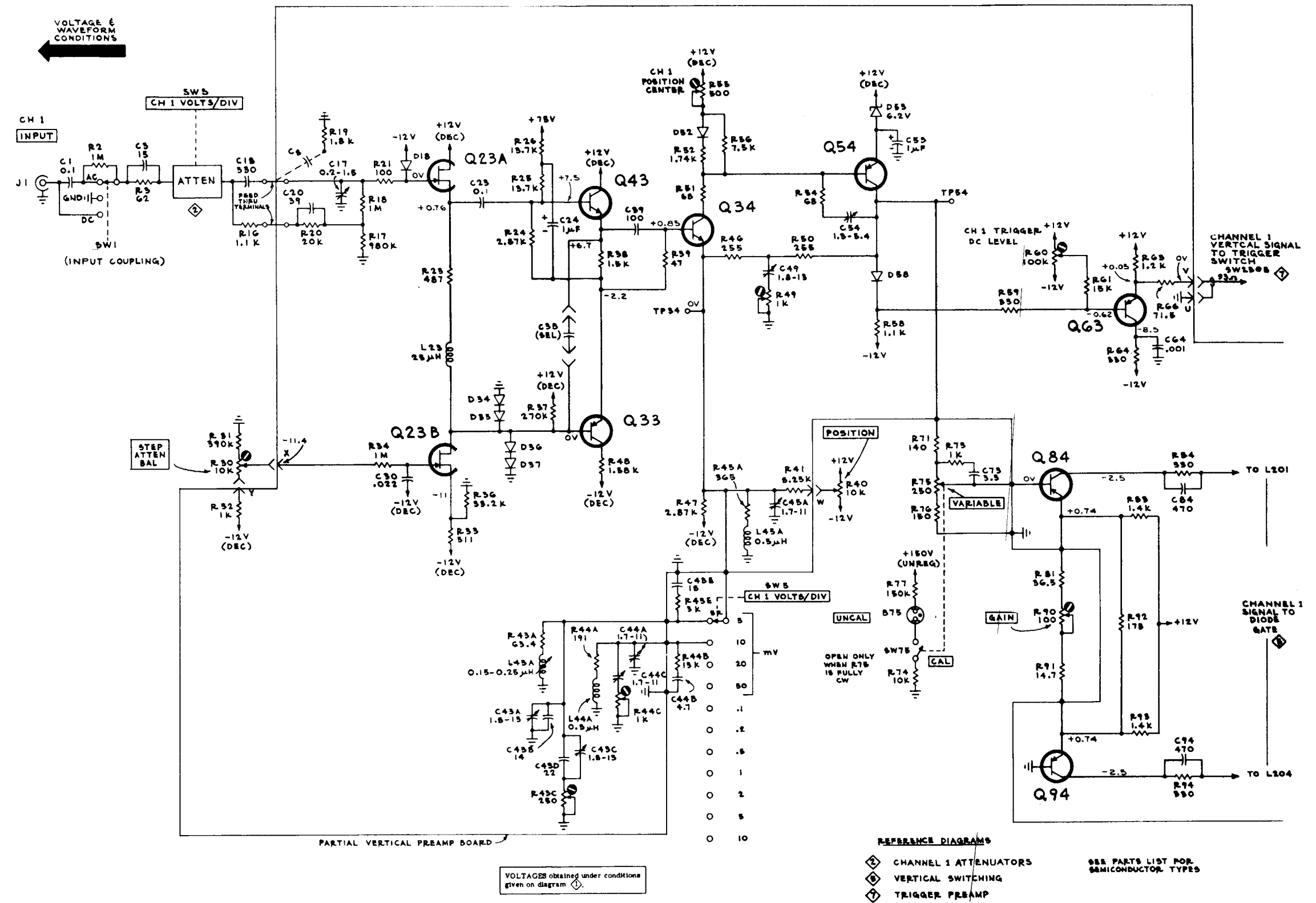
FIG. FO-11. CHANNEL 1 VERTICAL PREAMP (S/N 20,000 & UP)
