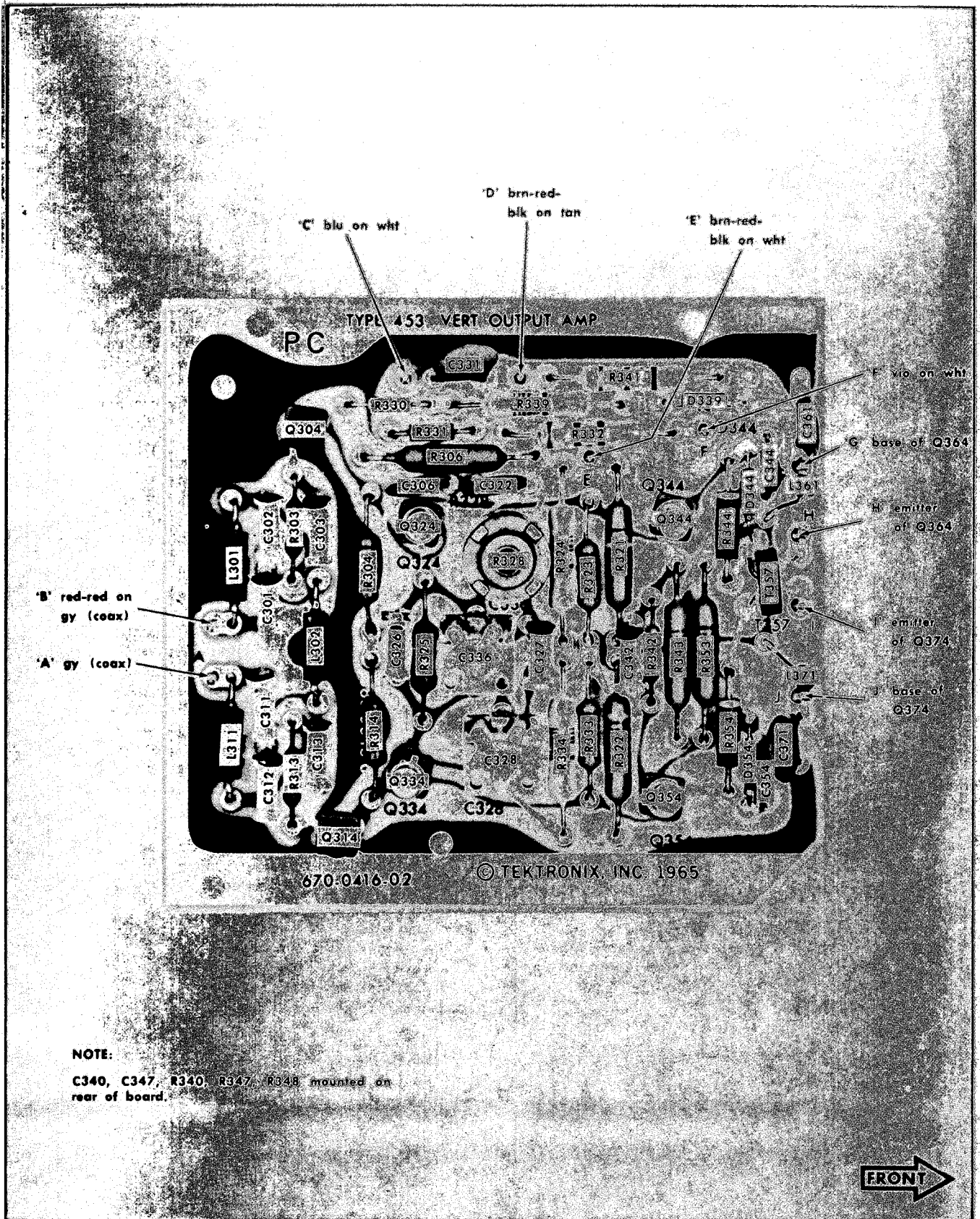
Fig. 4-8. Vertical Output Amplifier circuit board.
