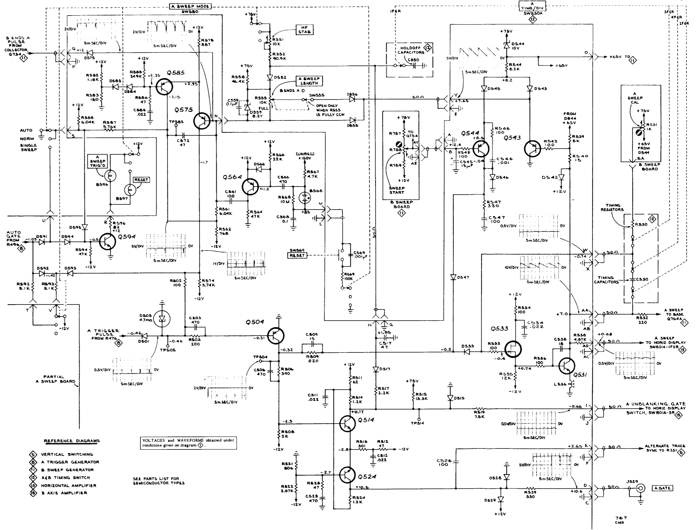
FIG. FO-19 A SWEEP GENERATOR (S/N 20,000 & UP)
