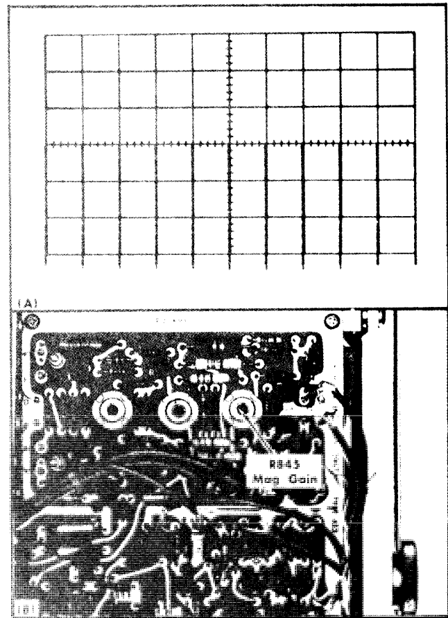
Fig. 6-40. (A) Typical CRT display showing correct magnified gain; (B) location of Mag Gain adjustment (B Sweep circuit board).
