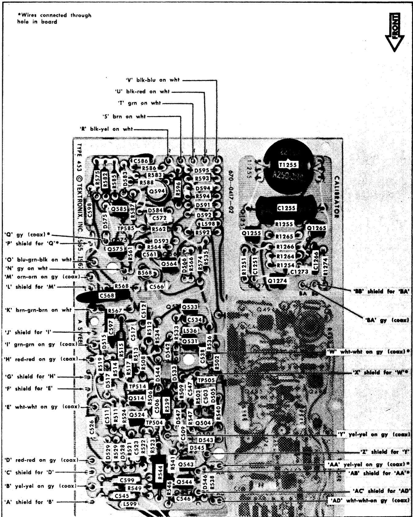
Fig. 4-11. Partial A Sweep circuit board. A Sweep Generator and Calibrator circuits shown.
