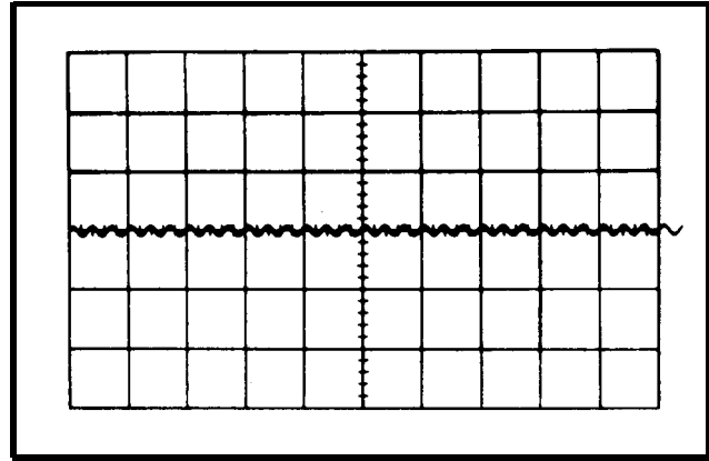
Fig. 6-35. Typical CRT display when checking low-frequency reject operation at 30 kilohertz.
