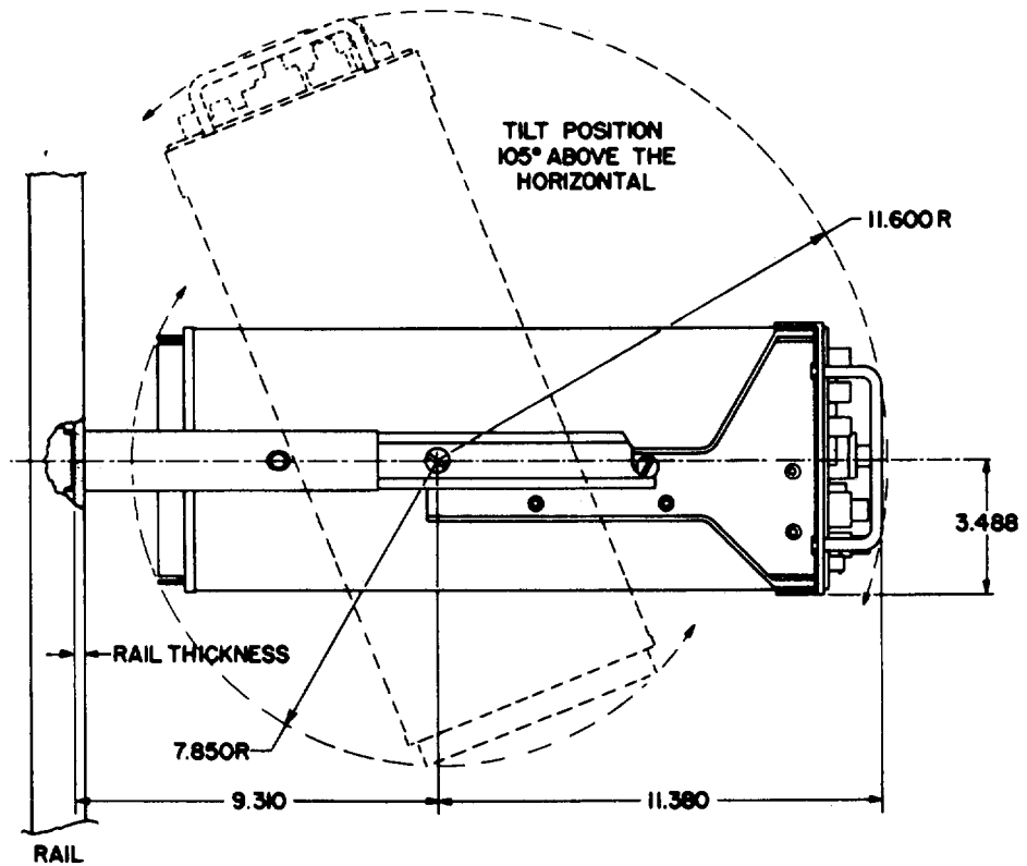
Figure 10-13. Pivoting Dimensions.
