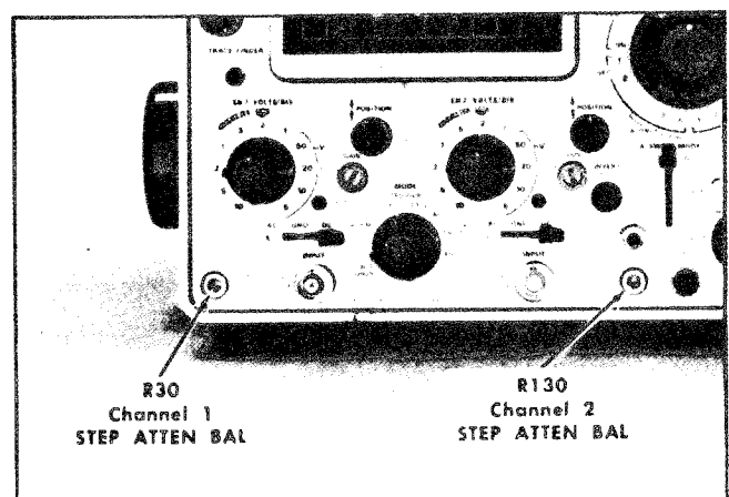
Fig. 6-14. Location of Channel 1 and 2 STEP ATTEN BAL adjustments (front panel).
