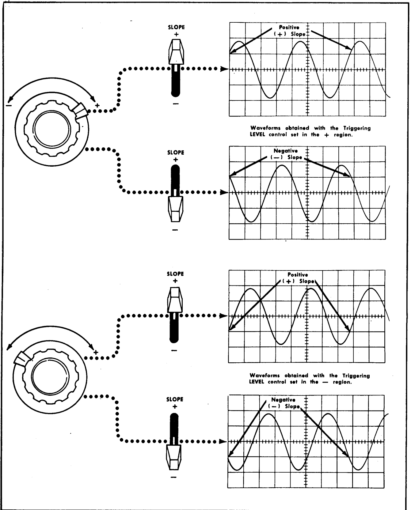
Fig. 2-8. Effects of Triggerring LEVEL control and SLOPE switch.
