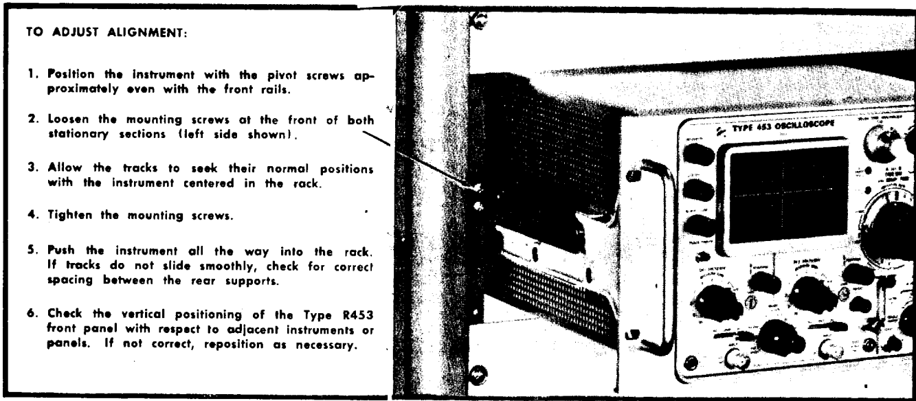
Fig. 10-10. Alignment adjustments for correct operation.
