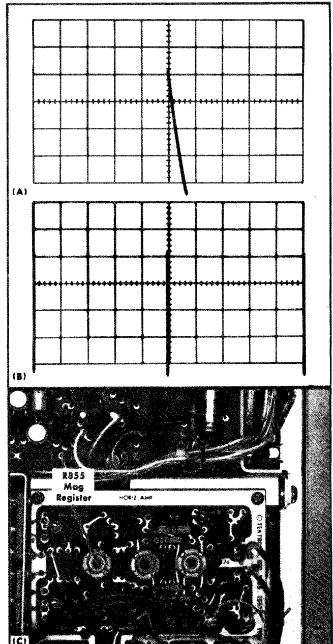
Fig. 6-41. Typical CRT display showing correct magnifier register. (A) MAG switch to X 10, (B) MAG switch set to OFF, (C) location of Mag Register adjustment (B Sweep circuit board).
