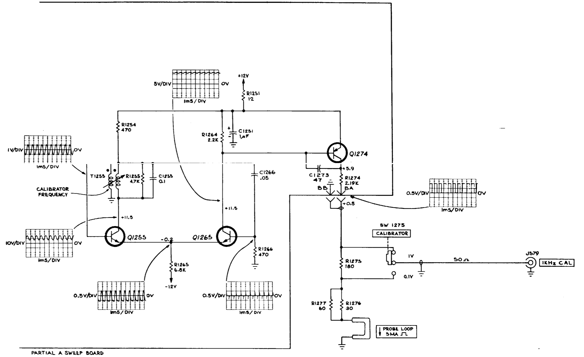
PARTIAL A SWEEP BOARD
