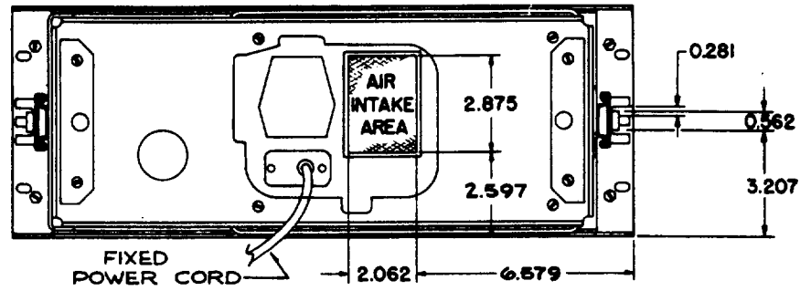
Figure 10-12. REAR VIEW
