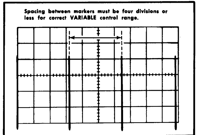
Fig. 5-23. Typical CRT display when checking A and B VARIABLE control range.
