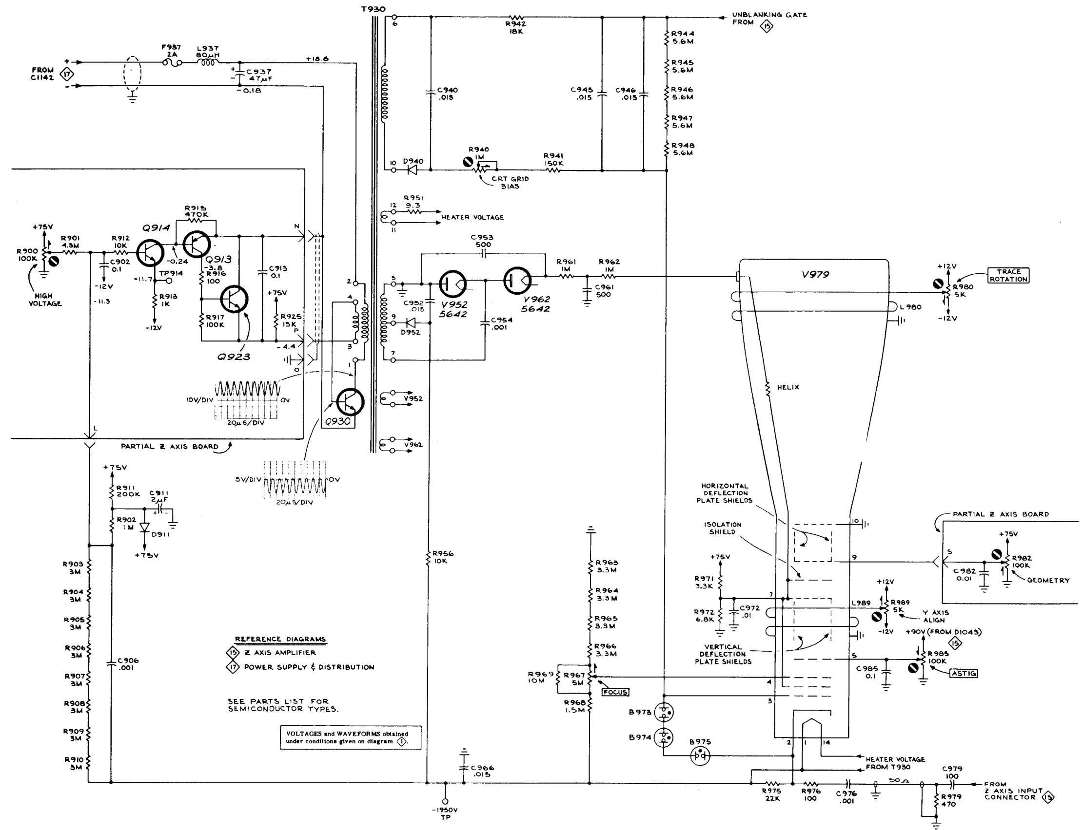
FIG. FO-26. CRT CIRCUIT (S/N 20,000 & UP) DON 668
