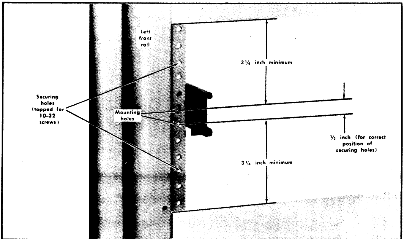
Fig. 10-6. Locating the mounting holes for the left stationary section. Same dimensions apply to right stationary section.
