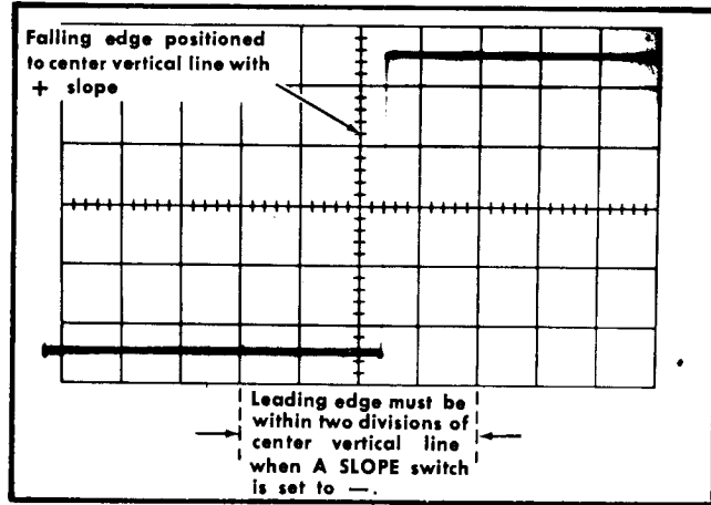
Fig. 5-29. Typical CRT display when checking calibrator duty cycle.
