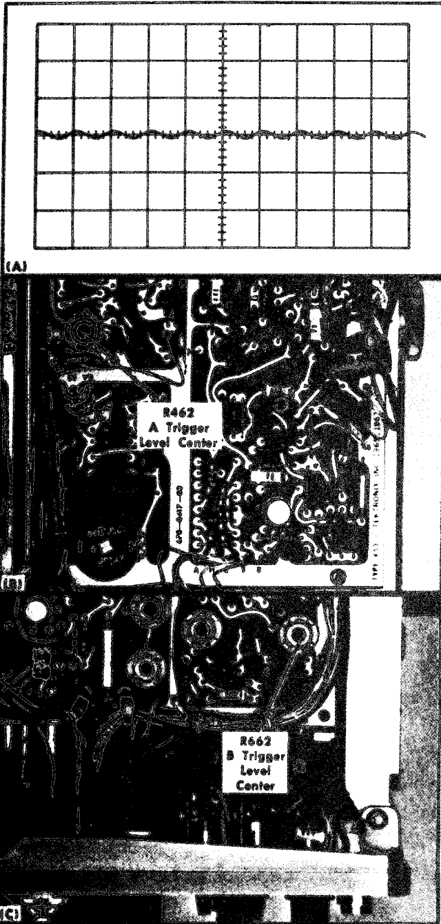
Fig. 6-29. (A) Typical CRT display when checking trigger level centering, (B) location of the A Trigger Level Center adjustment (A Sweep circuit board), (C) location of B Trigger Level Center adjustments of (B Sweep circuit board).
