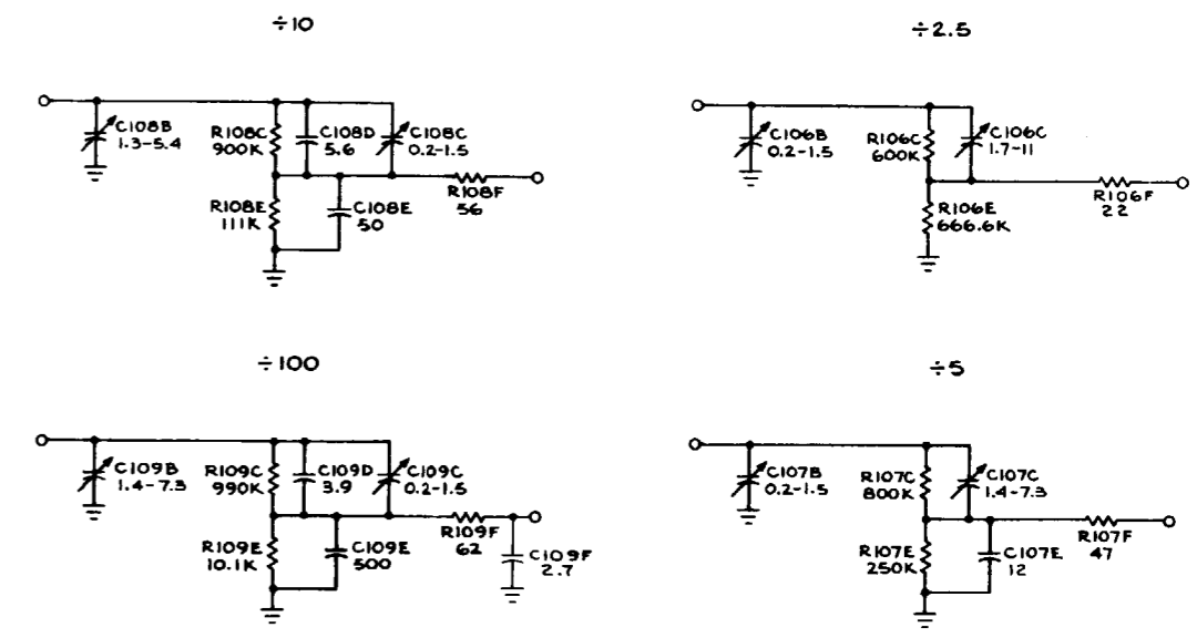
REFERENCE DIAGRAM CHANNEL 2 VERTICAL PREAMP
