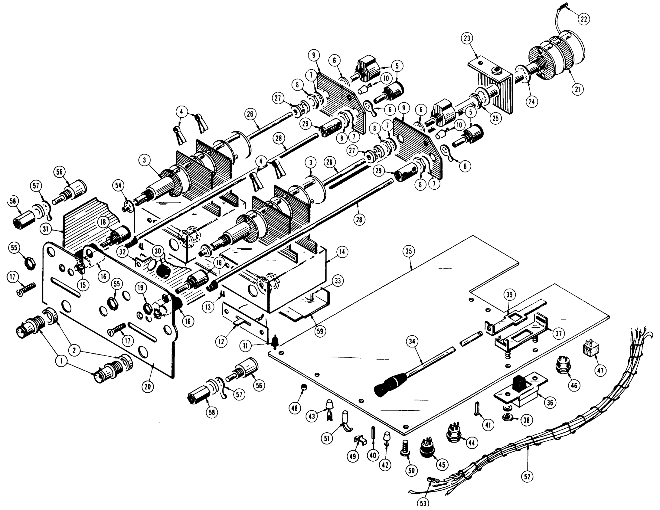
FIG. FO-2 ATTENUATOR PREAMPLIFIER ASSEMBLY
