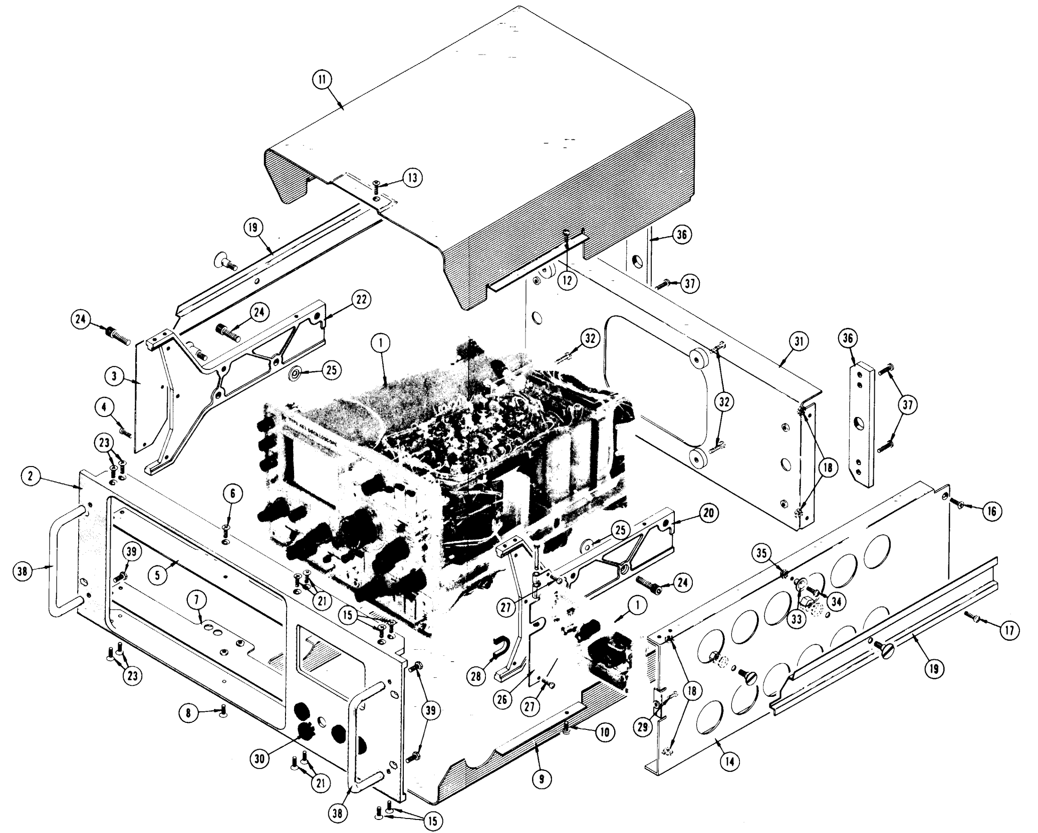
FIG. FO-8 R453 MECHANICAL PARTS
