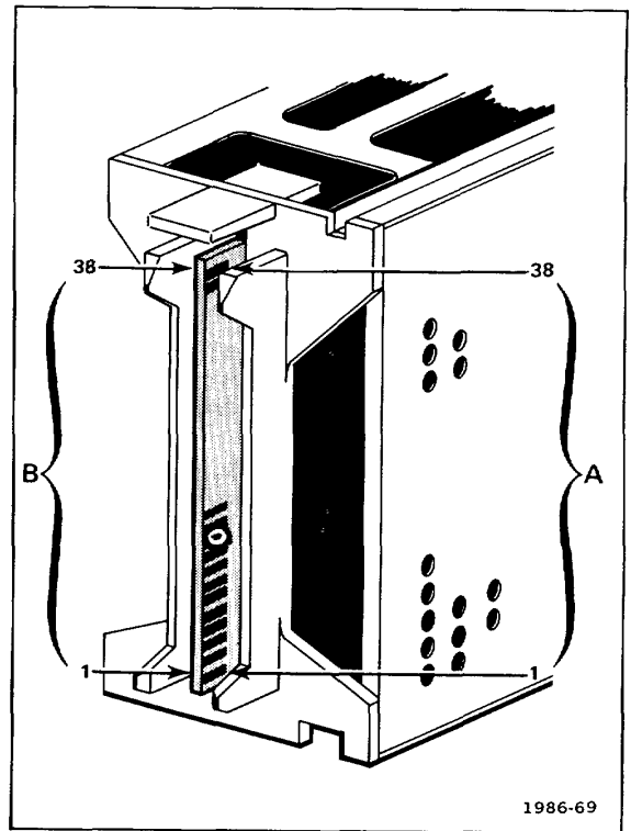
Fig. 4-5. Location of pin numbers of Interface connector.
