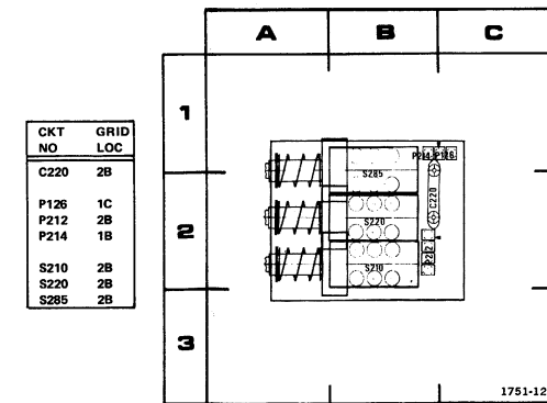
Fig. 8-4. A5—Delayed Triggering Switch Circuit Board.
