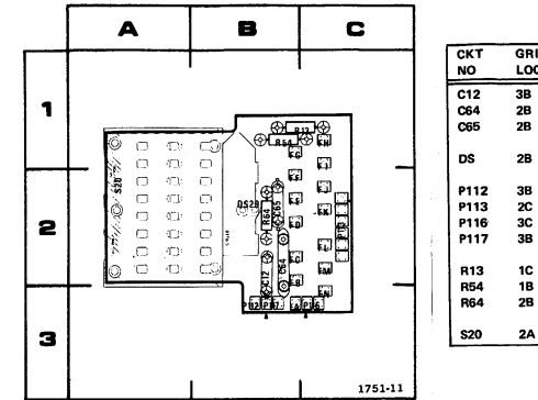
Fig. 8-3. A3—Coupling Switch Circuit Board.
