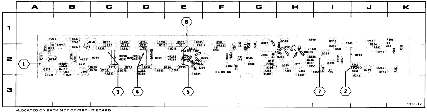
Fig. 8-11. A9—Delayed Trigger Circuit Board (SN B069999 & below).
