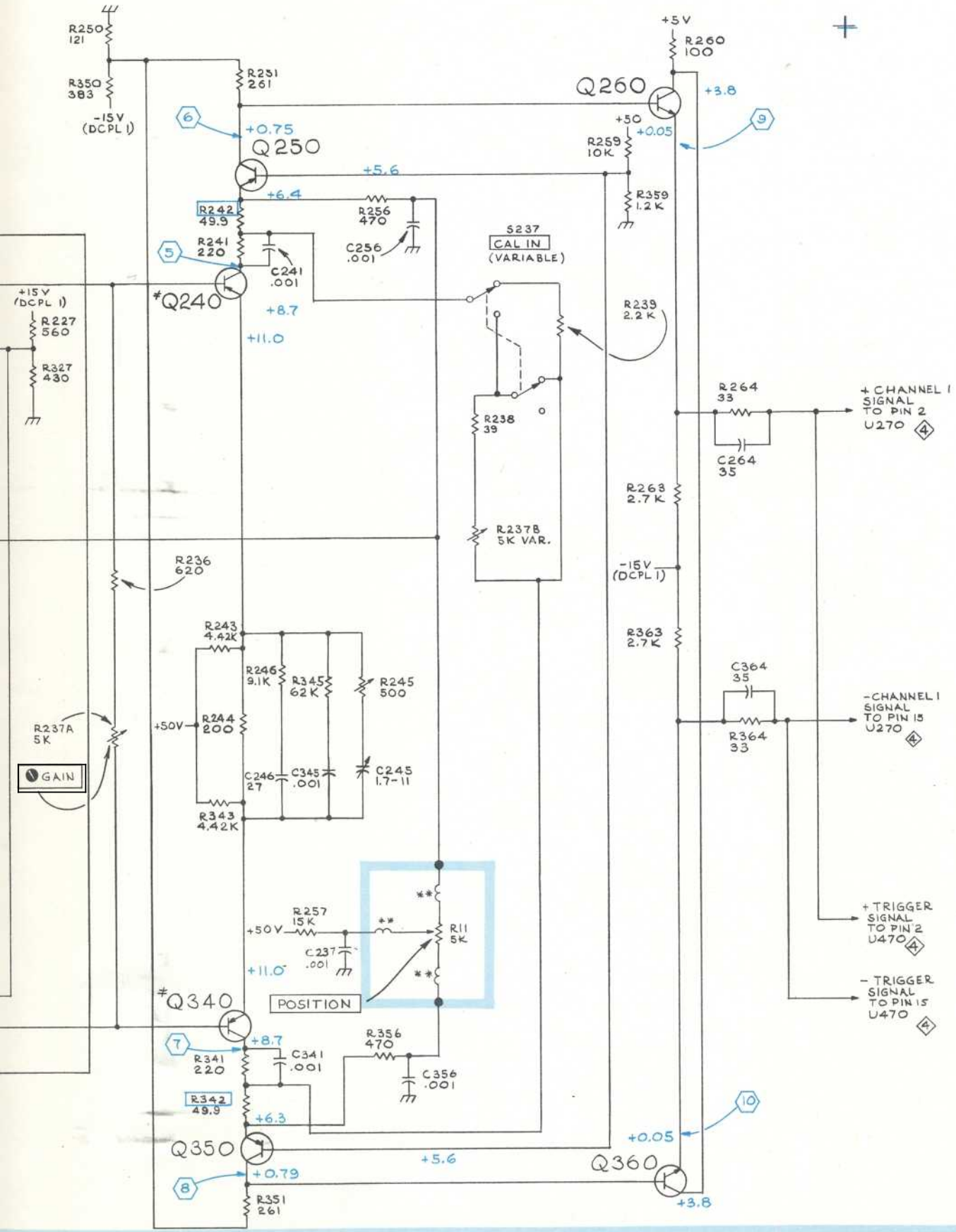
CHANNEL 1 INPUT AMPLIFIER SN B060000 - UP R.E.C. 474
