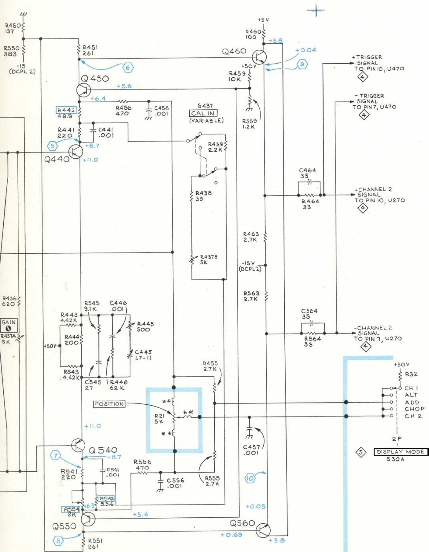
CHANNEL 2 INPUT AMPLIFIER 3 SNB060000 - UP
