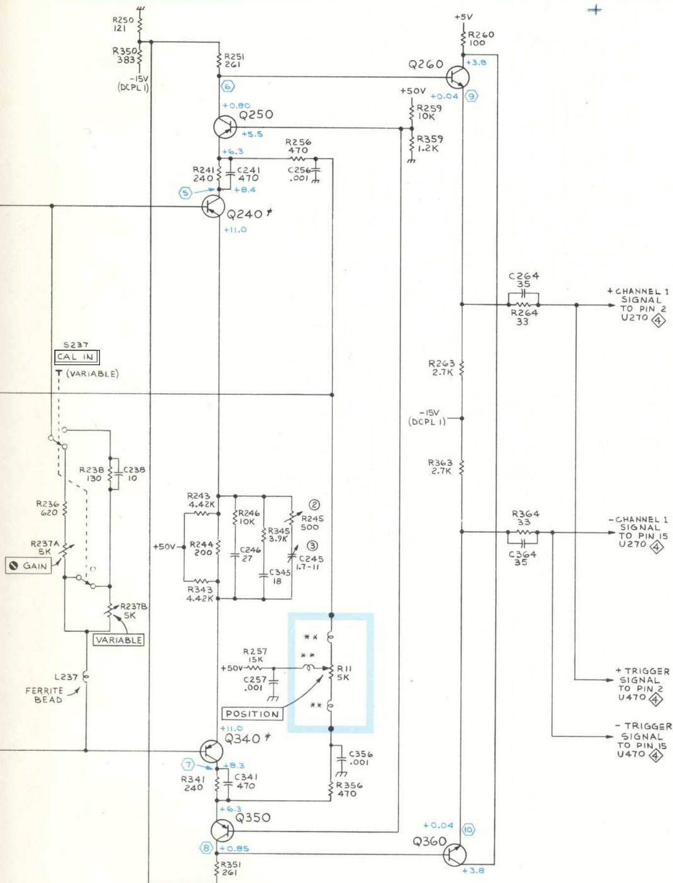
CHANNEL 1 INPUT AMPLIFIER 2 / hq BELOW SNB060000 REV. APR 1974
