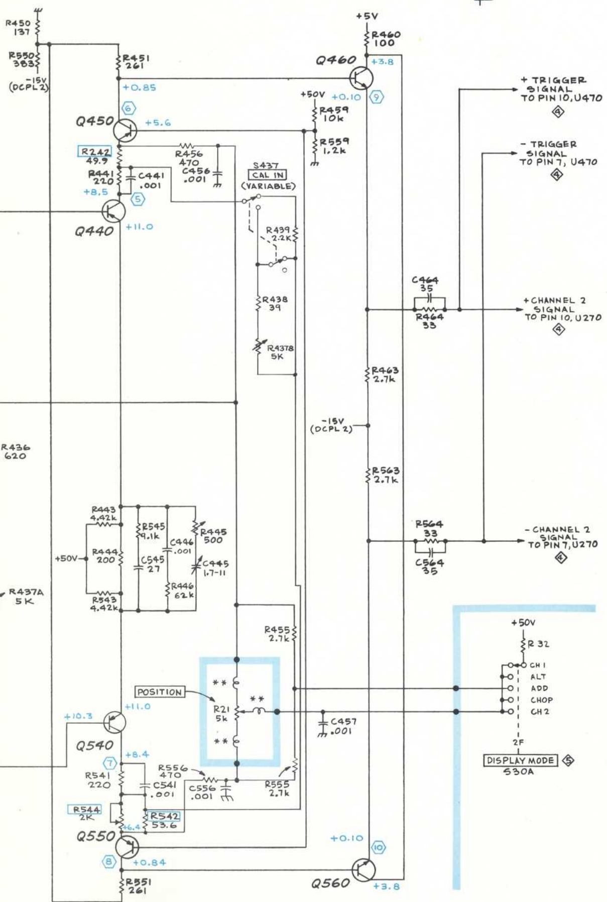
CHANNEL 2 INPUT AMPLIFIER
