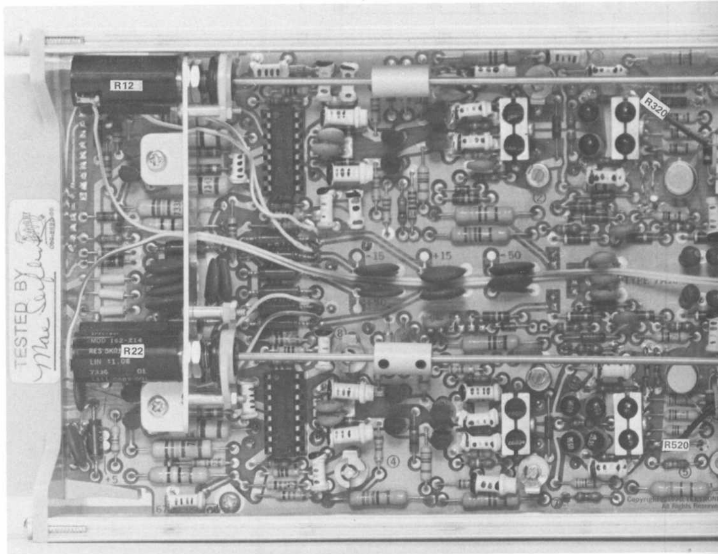
Fig. 7-1A. Amplifier Circuit Board Assembly, Option 6.
