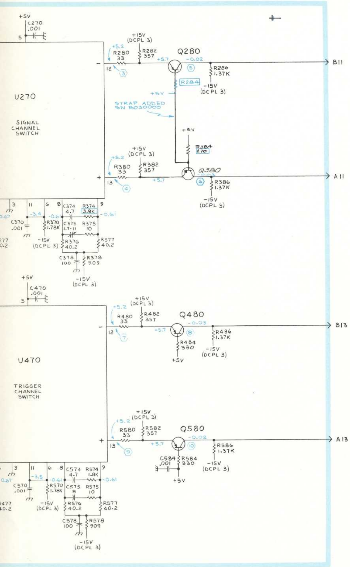
CHANNEL SWITCHES 4 mgf/hq REV. APR. 1974
