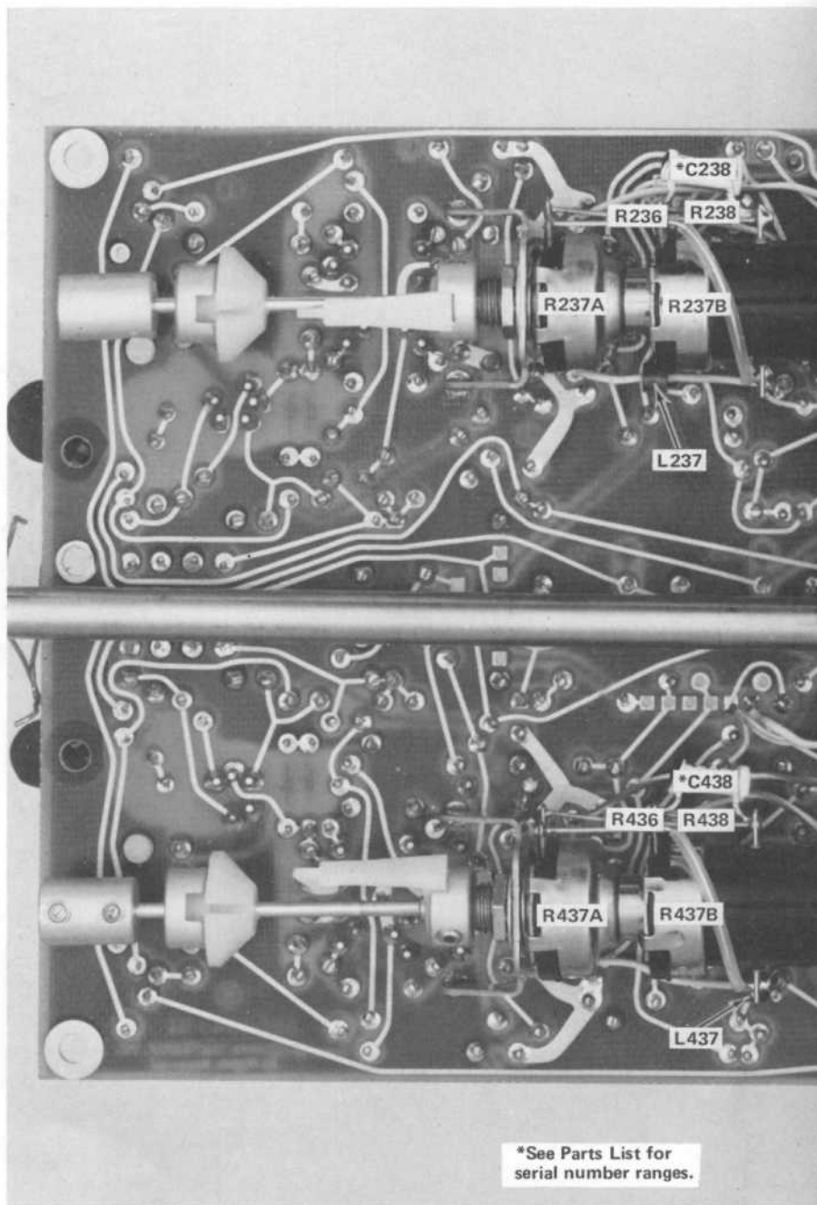
Fig. 7-2. A2 Amplifier Circuit Board
